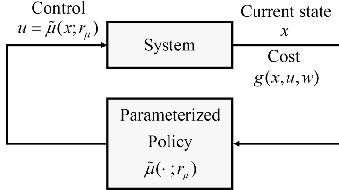
Figure 1.12: Direct policy optimization adjusts a parameterized policy using the closed-loop performance generated through interaction with the system.
