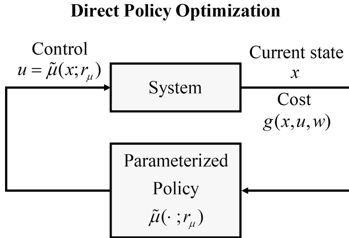
Figure 1.12: Direct policy optimization adjusts a parameterized policy using the closed-loop performance generated through interaction with the system.
