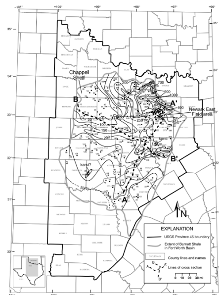
Figure 6. Map showing regional extent of Barnett Shale, thickness of Barnett Shale in selected wells, generalized regional isopachs of Barnett Shale, and lines of well-log cross sections AA' of Figure 9 and BB' of Figure 10. Contour intervals are 50 ft (15 m) for thicknesses from 0 to 300 ft (0 to 91 m) and 100 ft (30 m) for thicknesses from 300 to 1000 ft (91 to 305 m). Modified from Pollastro (2003).
