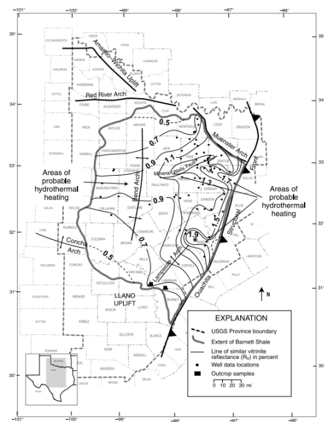
Figure 12. Map shows lines of equal thermal maturity as determined from mean vitrinite reflectance ( R_o ) of Barnett Shale. Based on data from Humble Geochemical Services, Humble, Texas. Areas of probable high hydrothermal heating and anomalously high R_o are also indicated (arrows).
