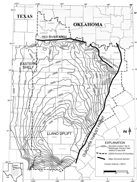
Figure 5. Generalized structure contour map, top of Ellenburger Group, Fort Worth Basin–Bend arch area of north-central Texas. Data interpreted from subsurface log and IHS well-history database (IHS Energy, 2003).
