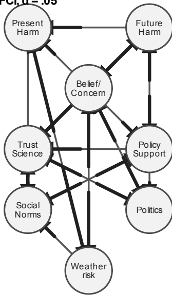
A FCI, \alpha = .05
