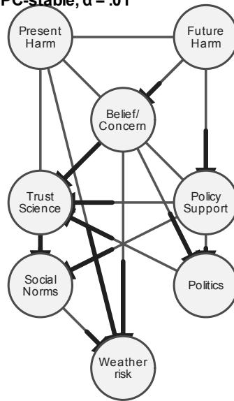
D PC-stable, \alpha = .01
