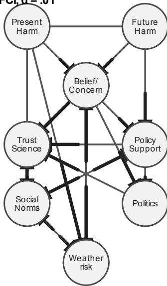
C FCI, \alpha = .01
