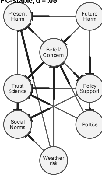
B PC-stable, \alpha = .05
