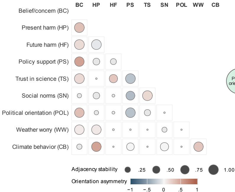
A FCI bootstrap stability
