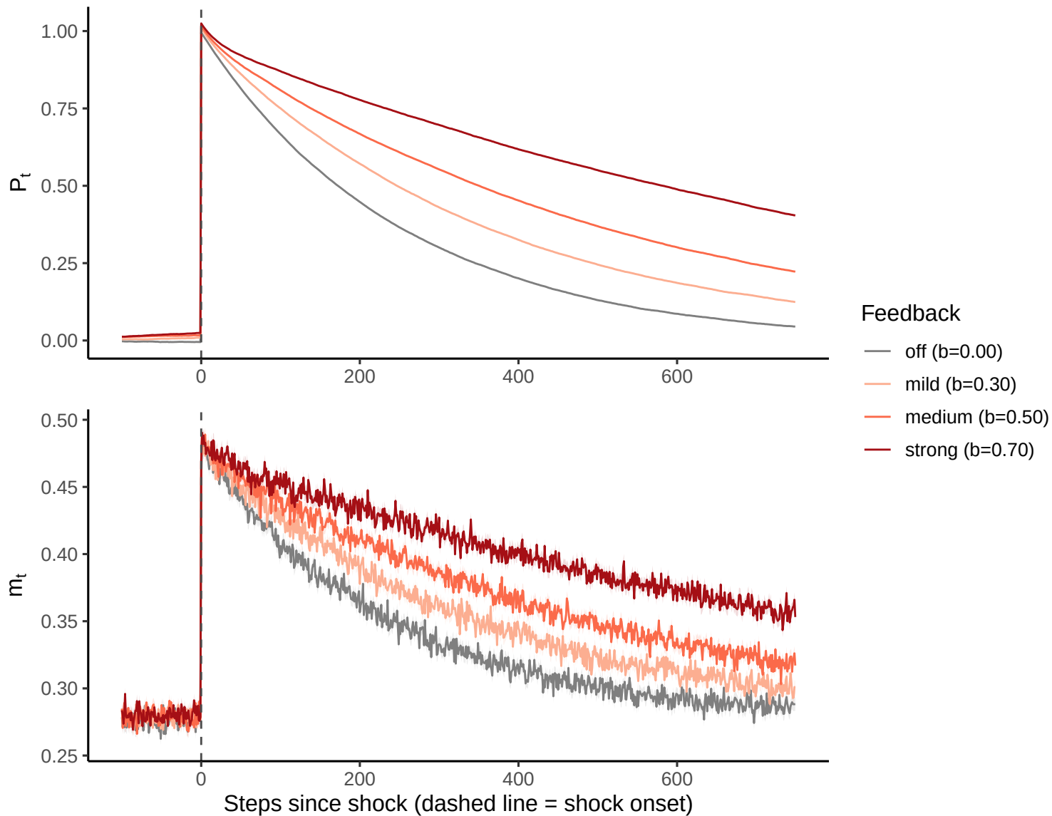
Simulation 3: stress and recovery across feedback strengths
