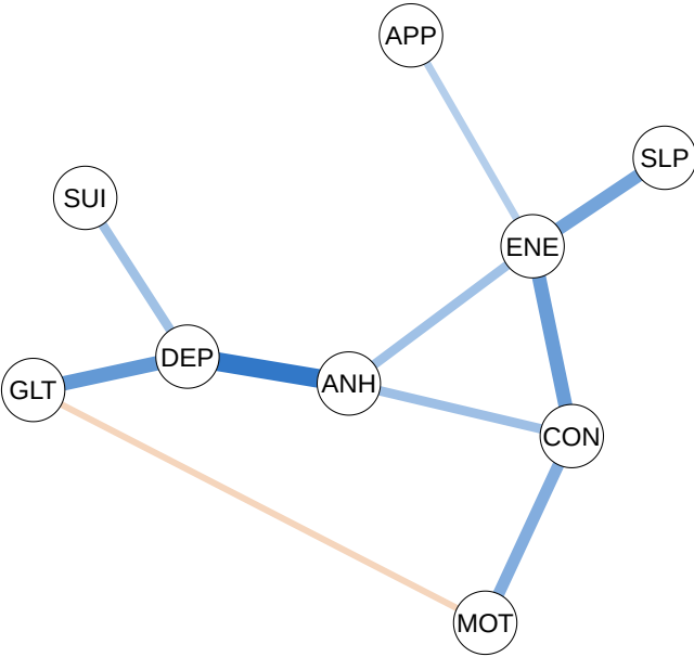
(B) Estimated network, fixed P
