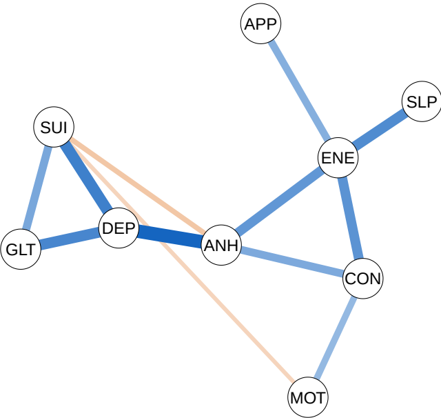
(C) Estimated network, P omitted
