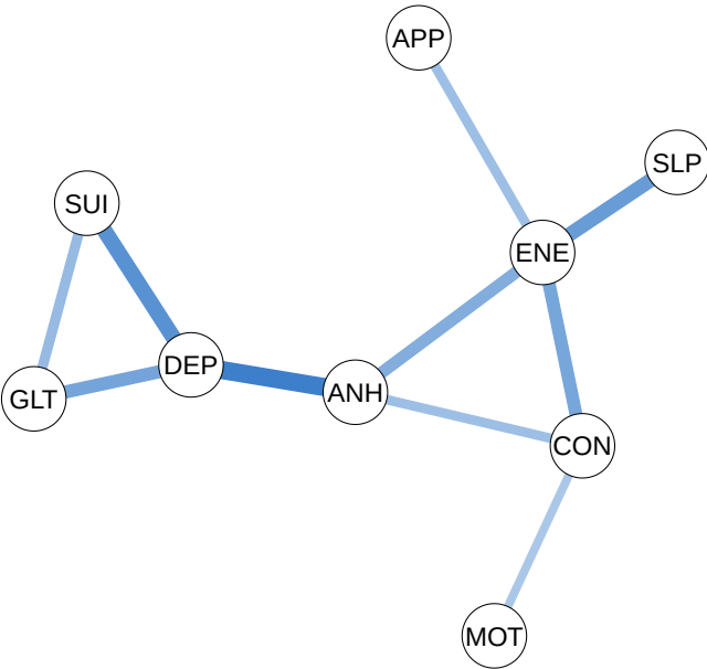
(D) Estimated network, P included
