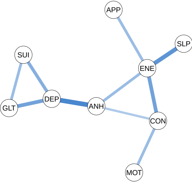
(A) True coupling
