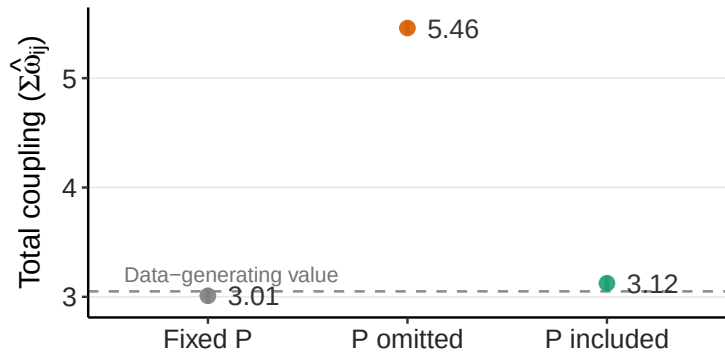
(E) Estimated total coupling
