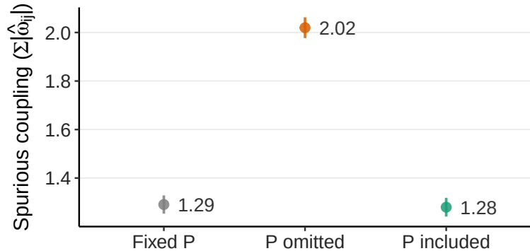
(F) Spurious coupling among uncoupled pairs
