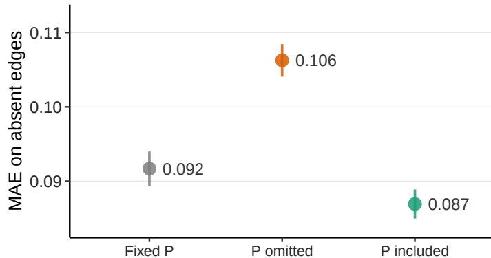
(E) Error on absent edges
