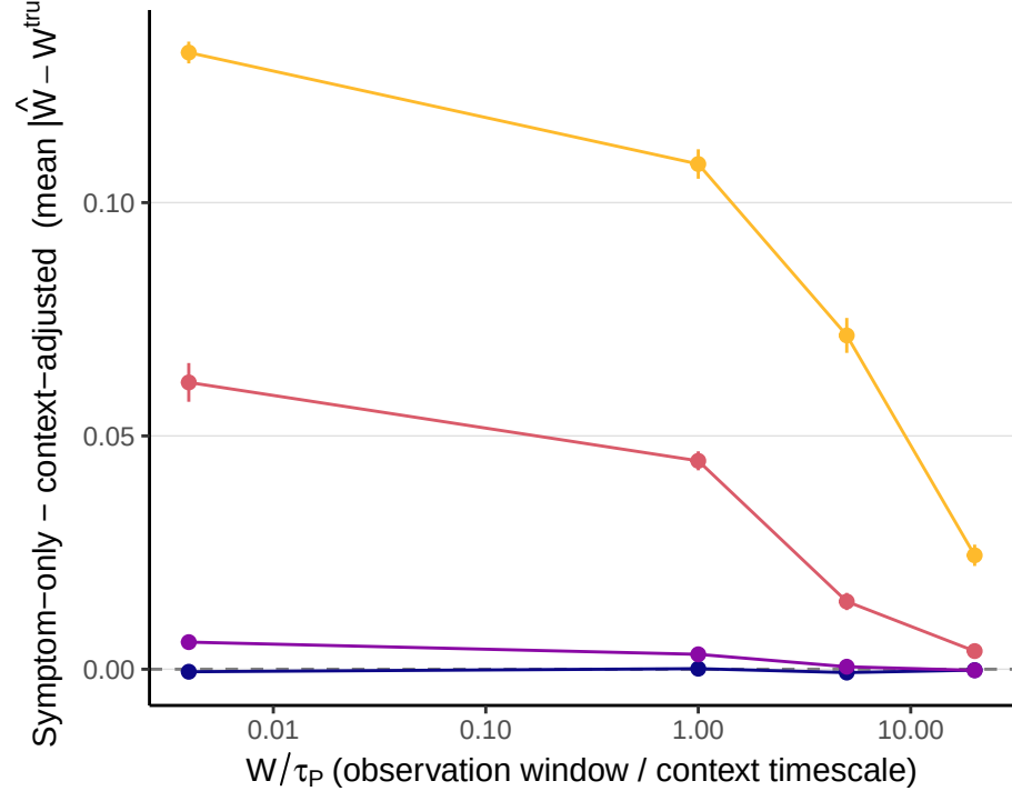
(C) Recovery-error bias vs. observation window
