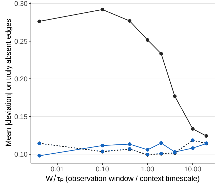
(C) Absent-edge deviation
