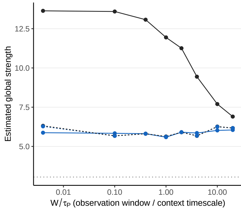
(B) Global strength
