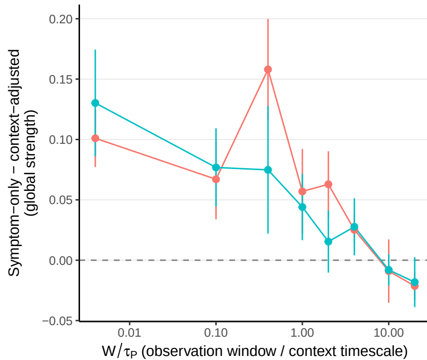
(B) Omitted-context bias vs. observation window
