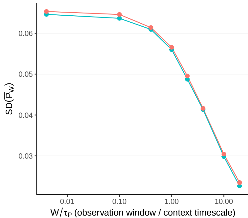
(A) Effective SD of \bar{P}_W
