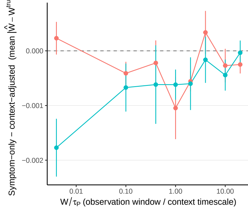
(C) Recovery-error bias vs. observation window
