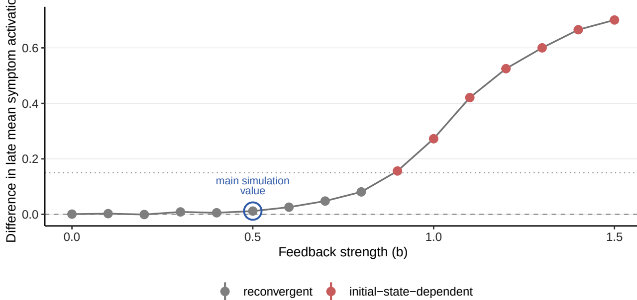
(C) Initial-state dependence emerges at higher feedback
