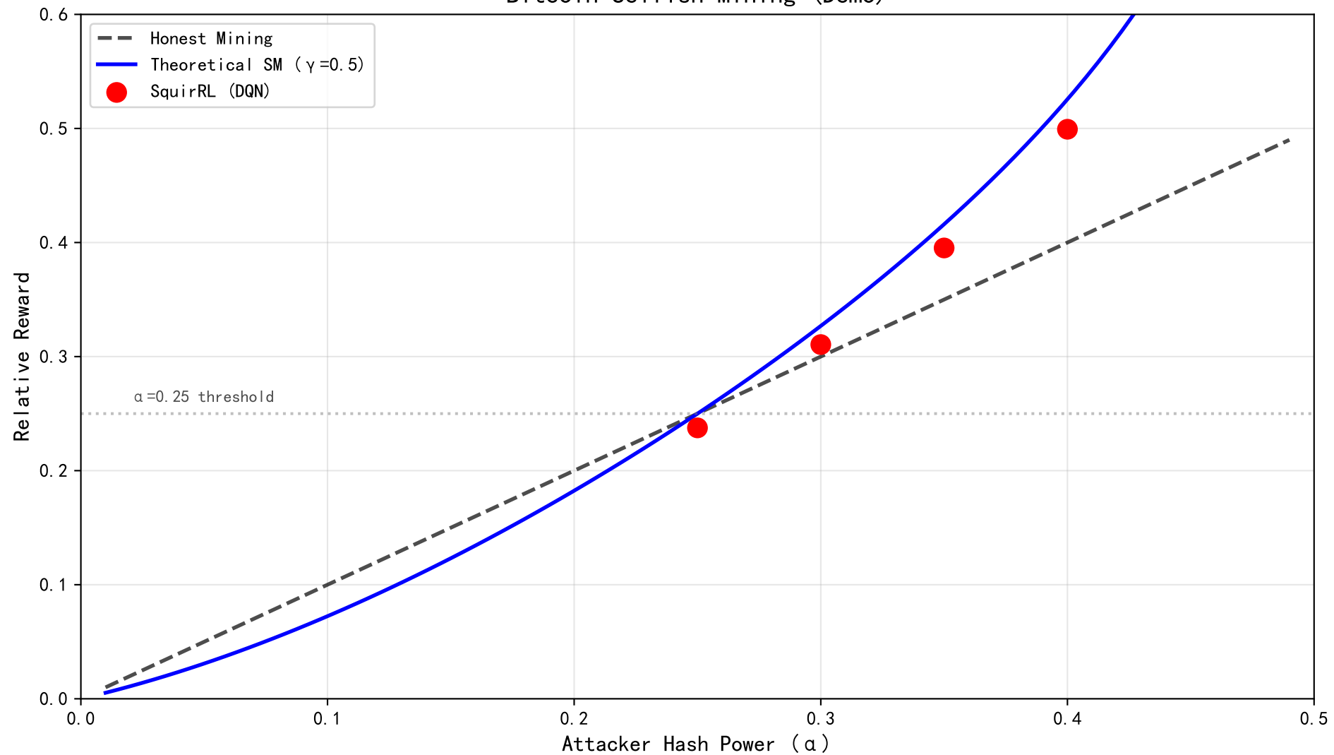
Bitcoin Selfish Mining (Demo)
