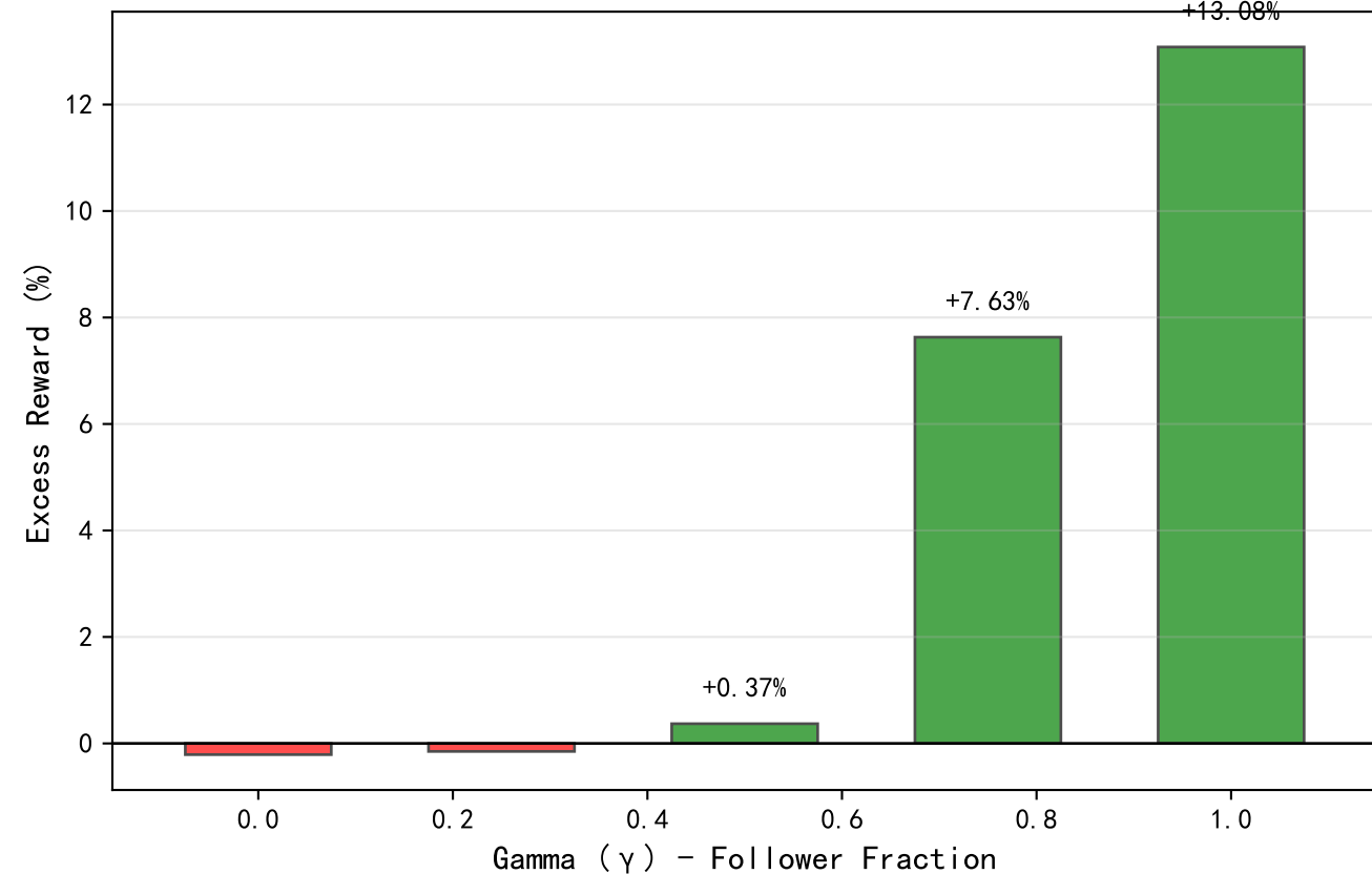
Excess Reward over Honest Mining (Bitcoin, \alpha=0.35 )
