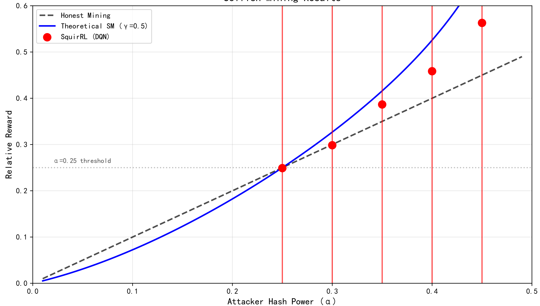
Selfish Mining Results
