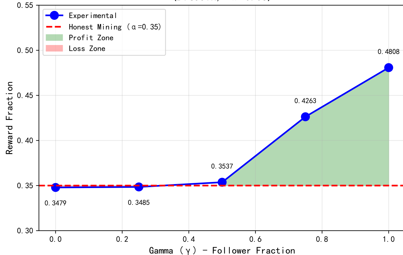
Selfish Mining Reward vs Follower Fraction (Bitcoin, \alpha=0.35 )
