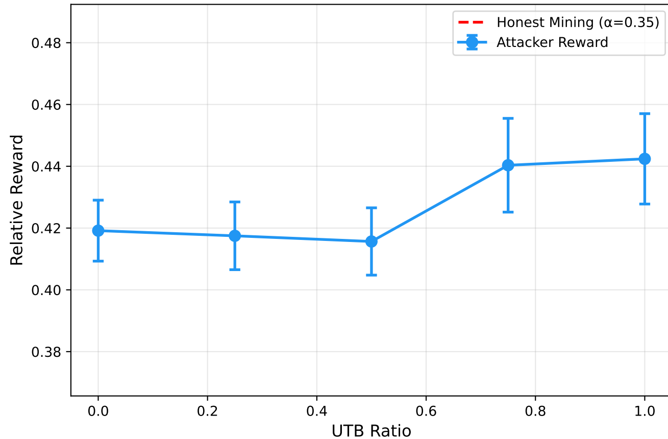
UTB Defense Effect ( \alpha=0.35 )
