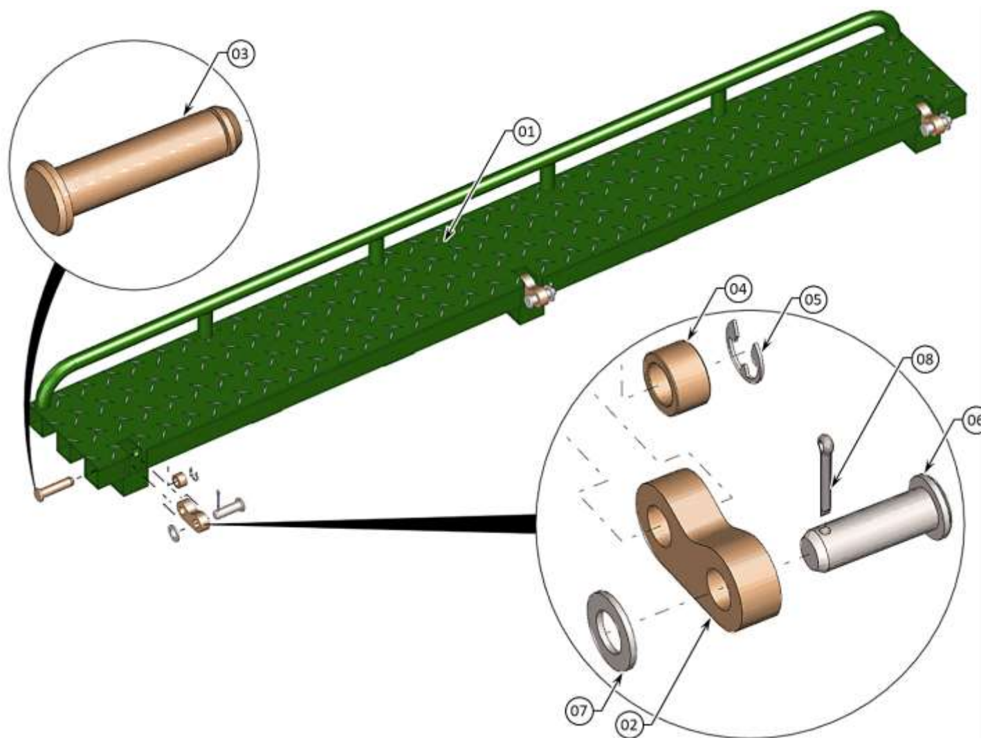
CURB ASSY (BCM) - VIEW 1
