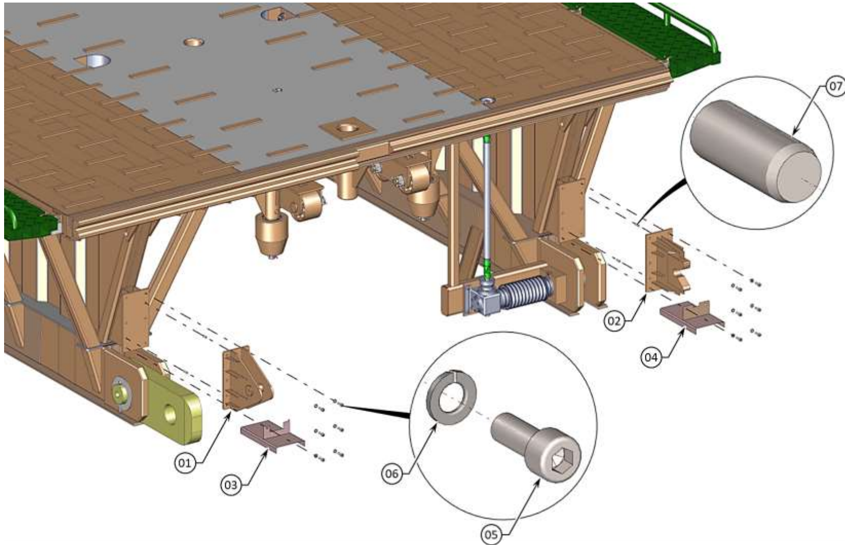
BRIDGE END MODULE ASSY - VIEW 1
