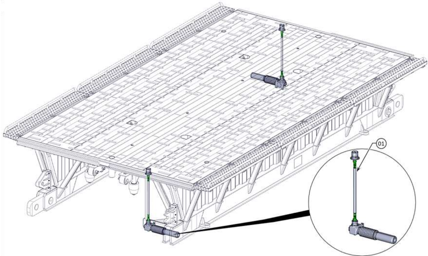
BRIDGE TO BRIDGE LOCKING MECHANISM (BCM)
