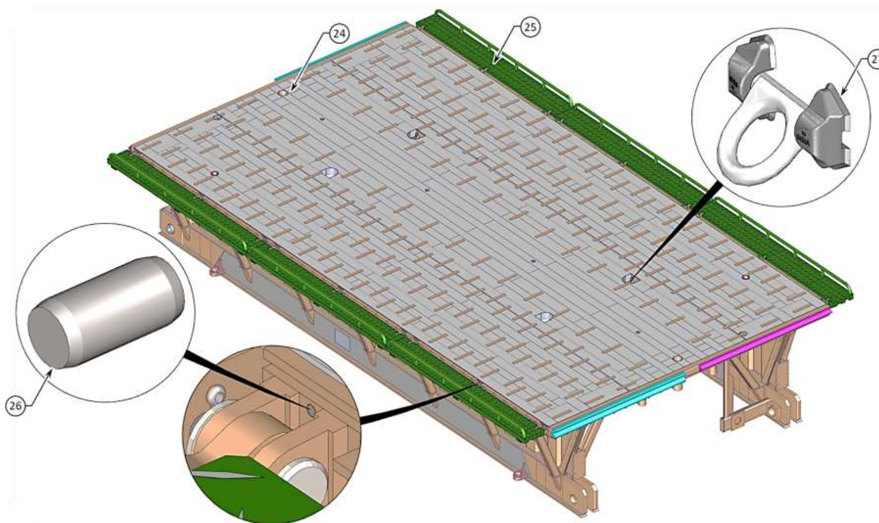
BRIDGE CENTRE MODULE ASSEMBLY - VIEW 5
