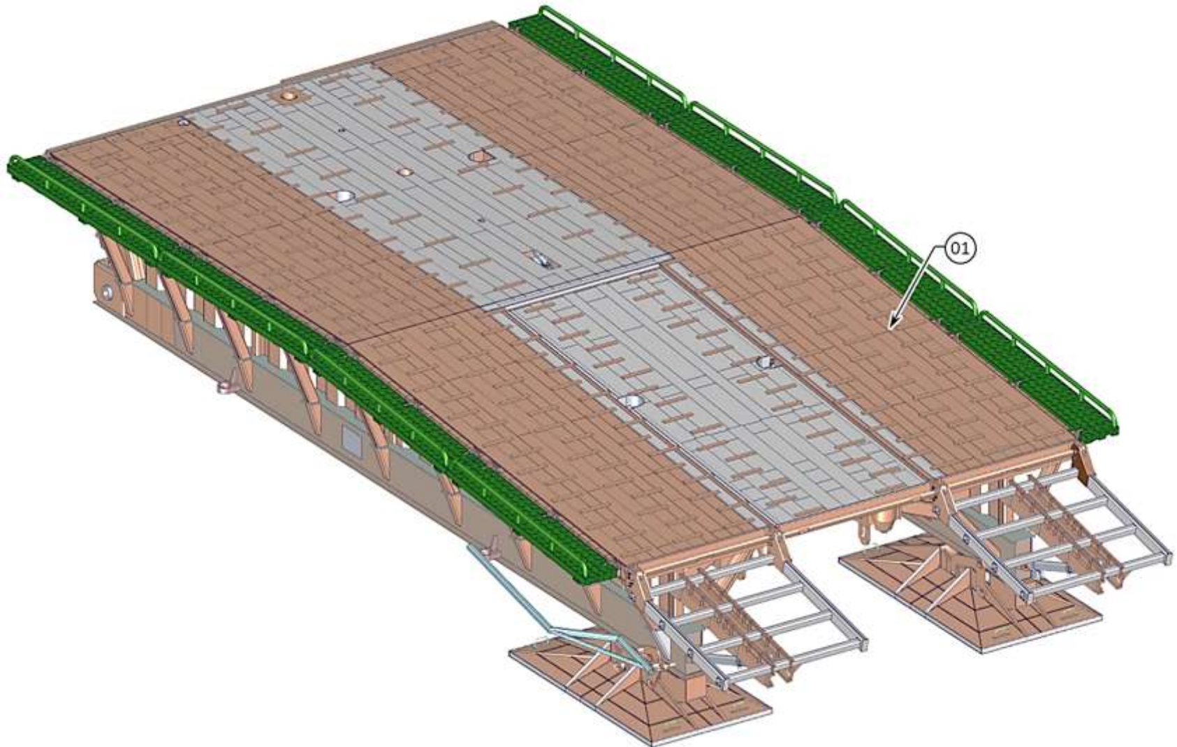
BRIDGE END MODULE ASSY
