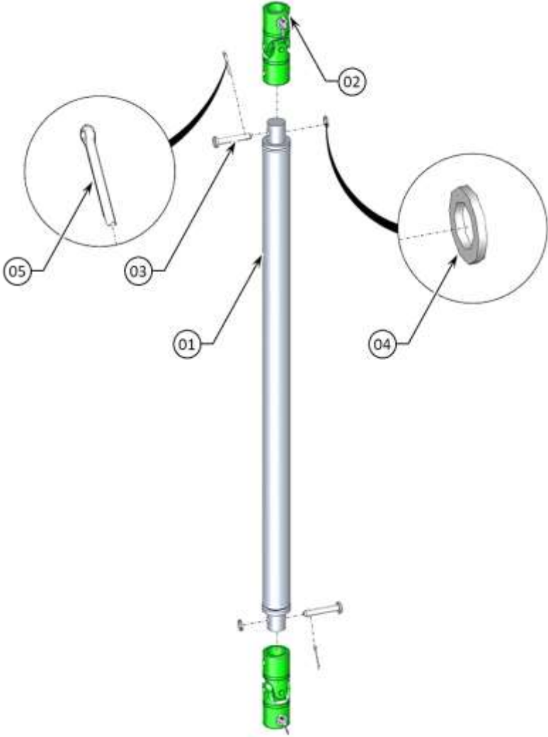
ASSEMBLY CONNECTING SHAFT (BRIDGE TO BRIDGE LOCKING MECHANISM) - VIEW 1
