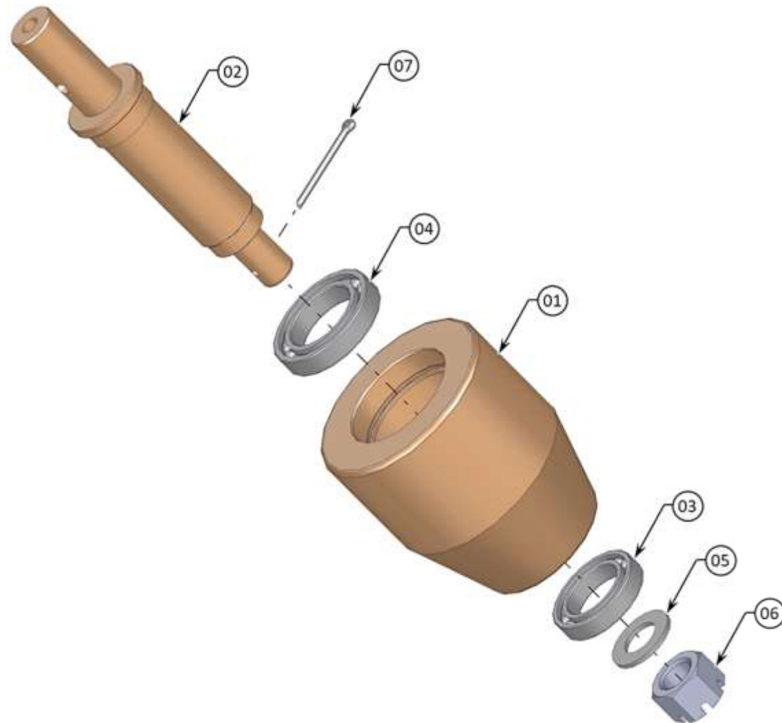
GUIDE ROLLER ASSEMBLY (BCM) - VIEW 1
