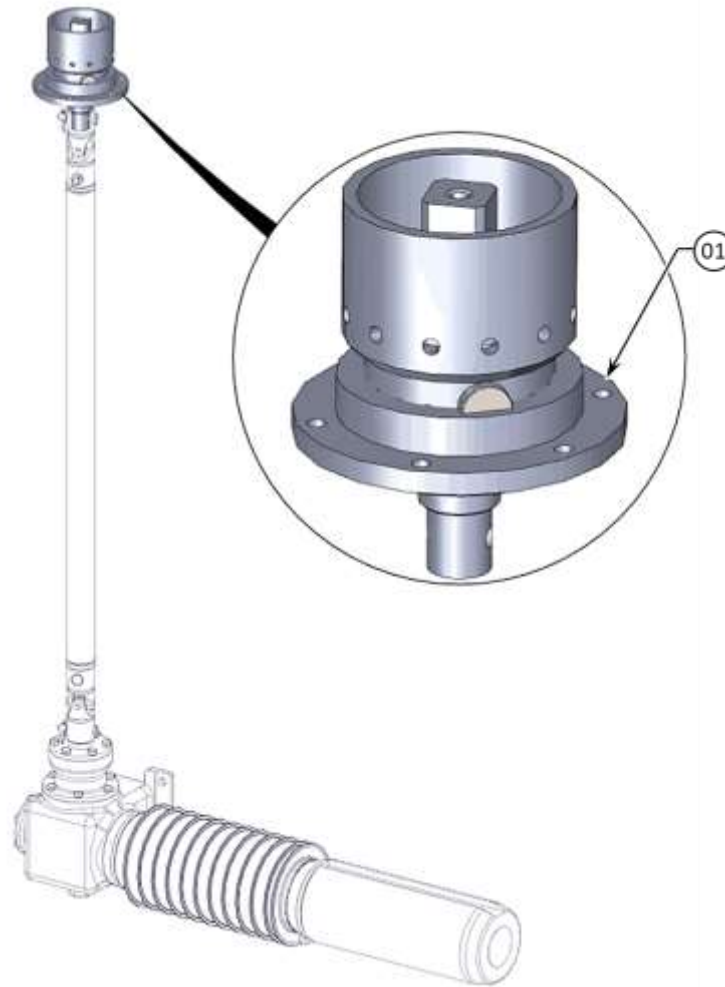
ASSY CONNECTING SHAFT WITH BEARING (BRIDGE TO BRIDGE LOCKING MECHANISM)
