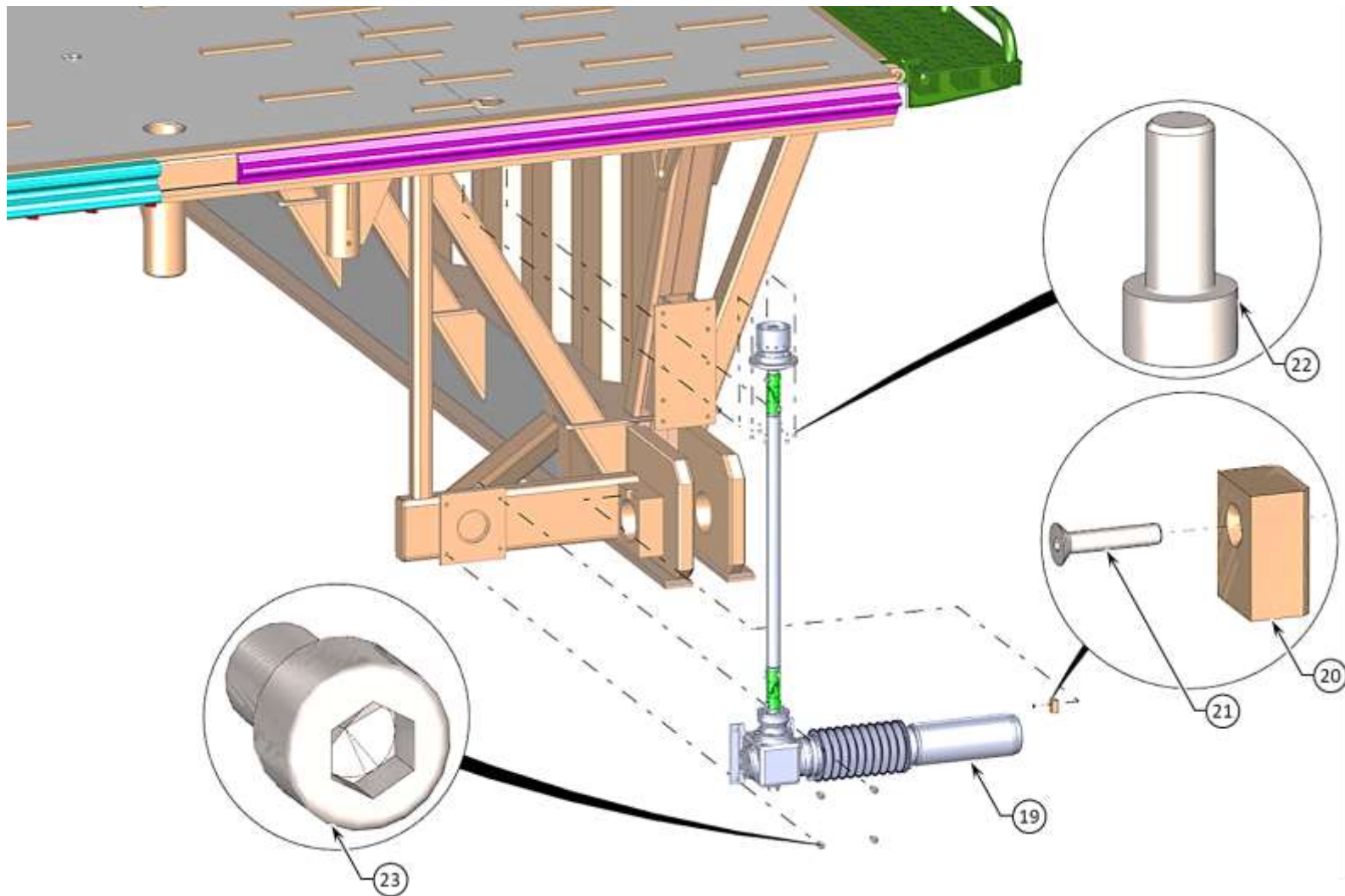
BRIDGE CENTRE MODULE ASSEMBLY - VIEW 4
