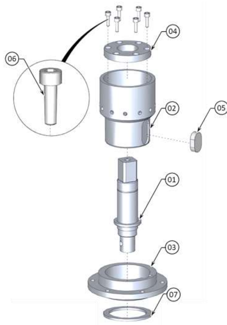
ASSY CONNECTING SHAFT WITH BEARING (BRIDGE TO BRIDGE LOCKING MECHANISM) - VIEW 1
