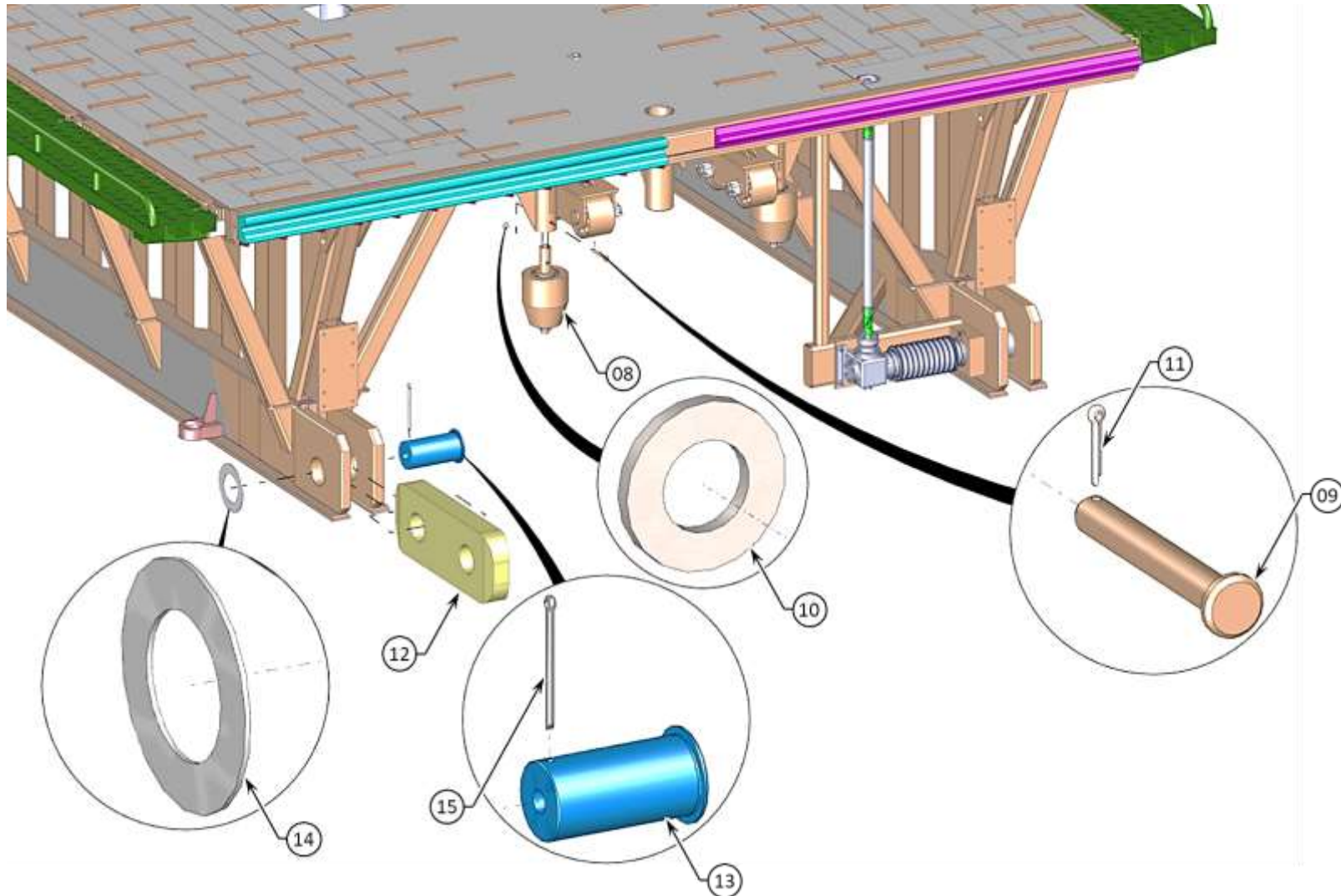
BRIDGE CENTRE MODULE ASSEMBLY - VIEW 2
