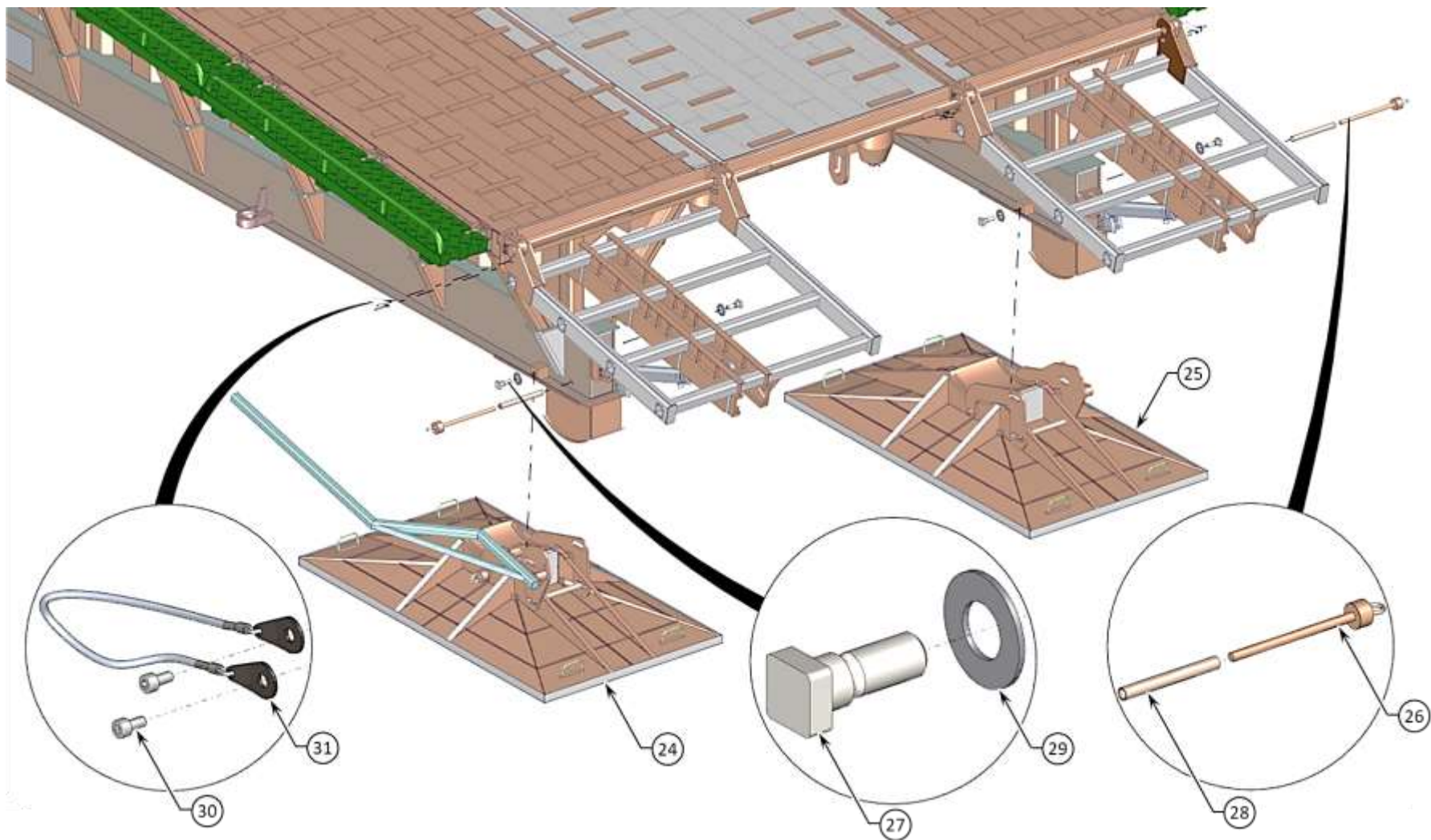
BRIDGE END MODULE ASSY - VIEW 4
