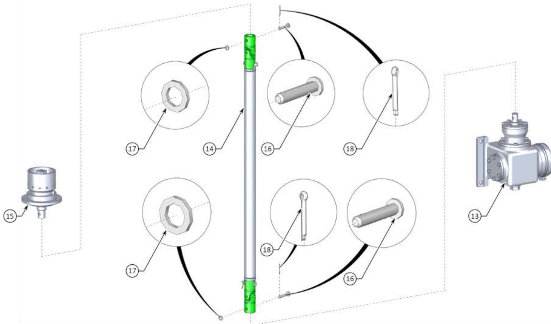
BRIDGE TO BRIDGE LOCKING MECHANISM (BCM) - VIEW 3
