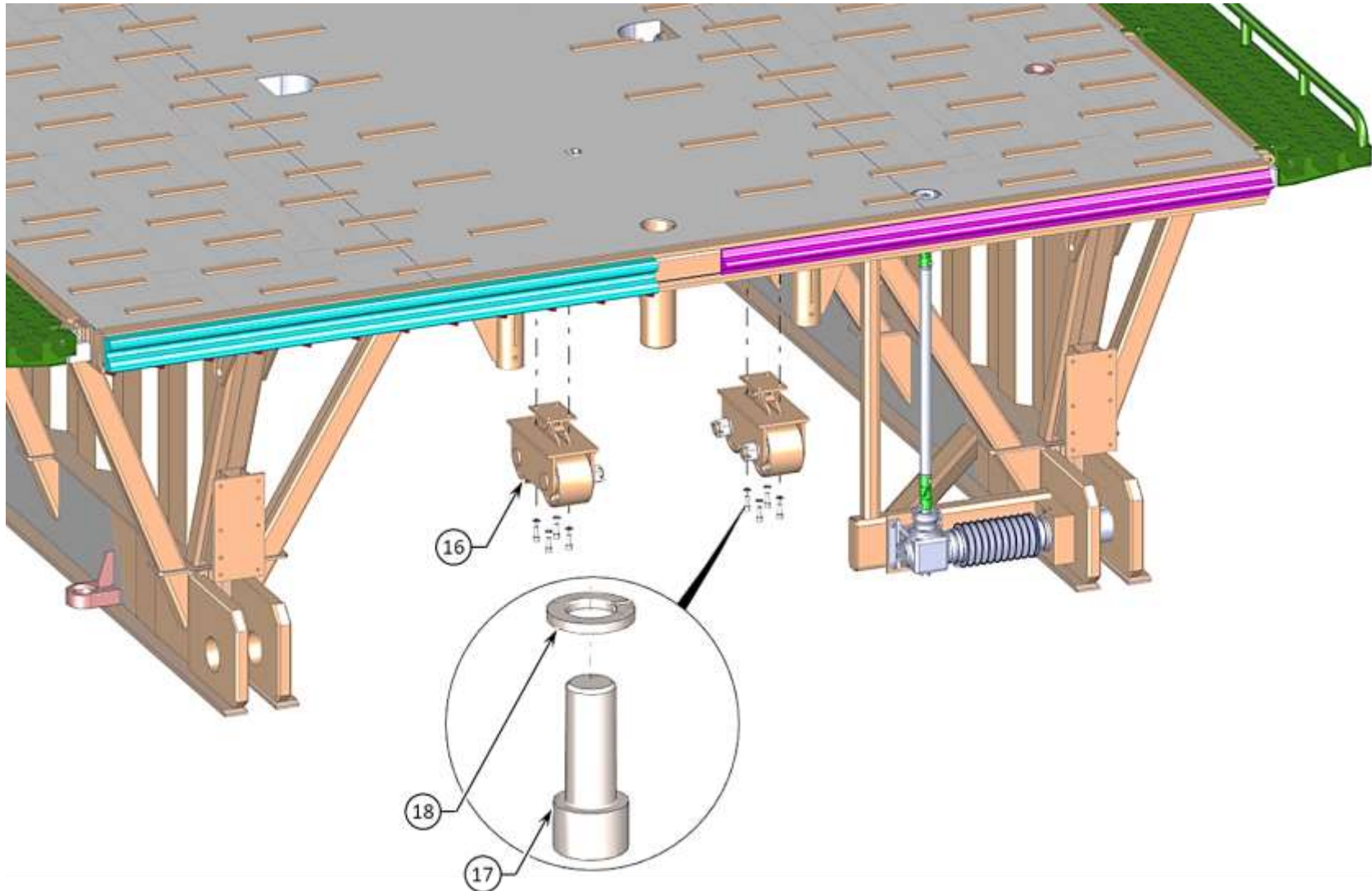
BRIDGE CENTRE MODULE ASSEMBLY - VIEW 3
