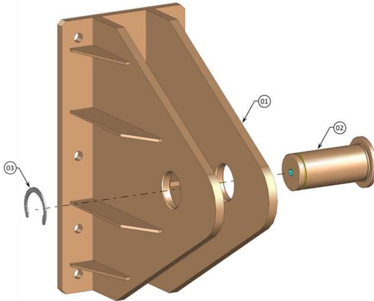
GUIDE BEAK MALE ASSEMBLY (BCM) - VIEW 1
