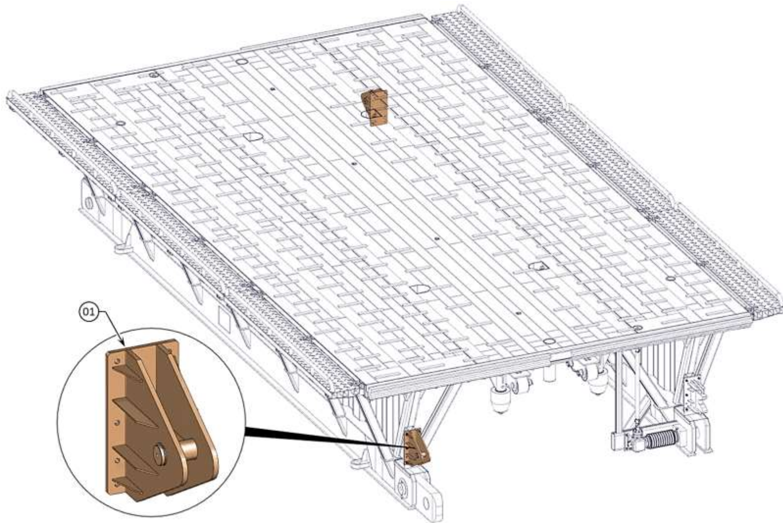
GUIDE BEAK MALE ASSEMBLY (BCM)
