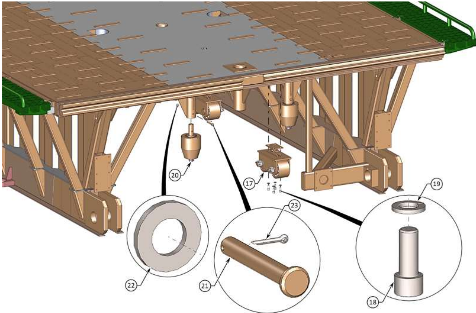
BRIDGE END MODULE ASSY - VIEW 3
