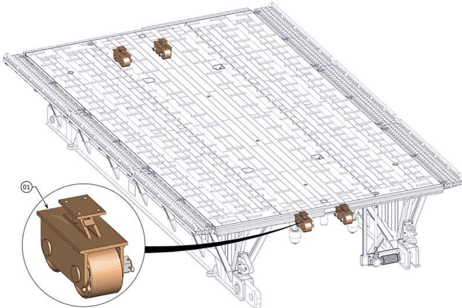
SUPPORT ROLLER ASSEMBLY (BCM)
