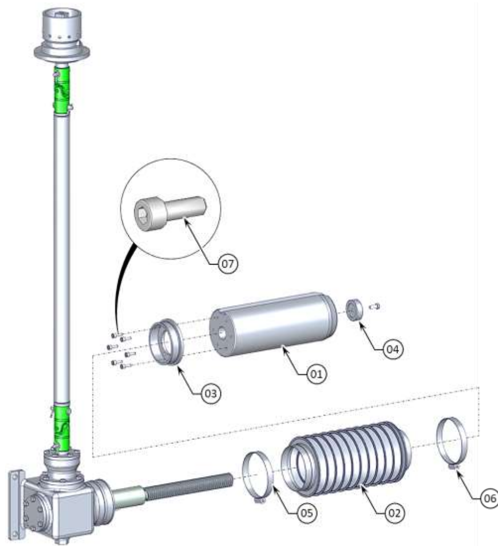
BRIDGE TO BRIDGE LOCKING MECHANISM (BCM) - VIEW 1
