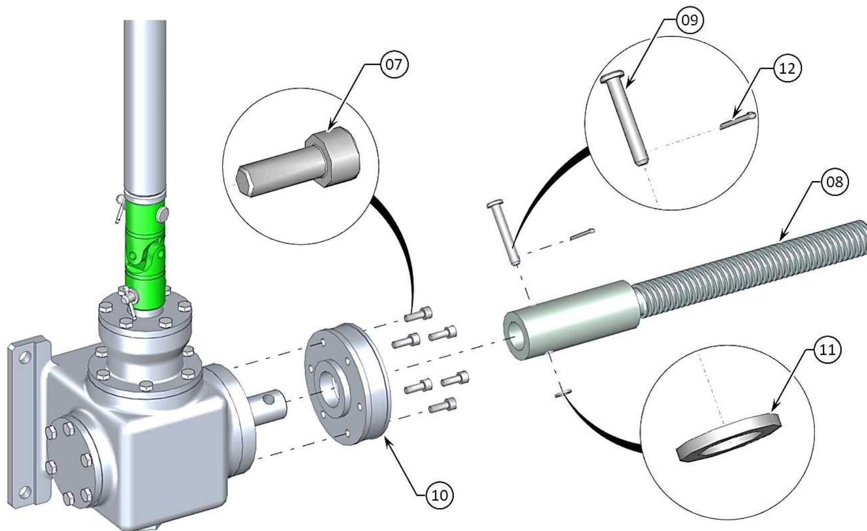
BRIDGE TO BRIDGE LOCKING MECHANISM (BCM) - VIEW 2
