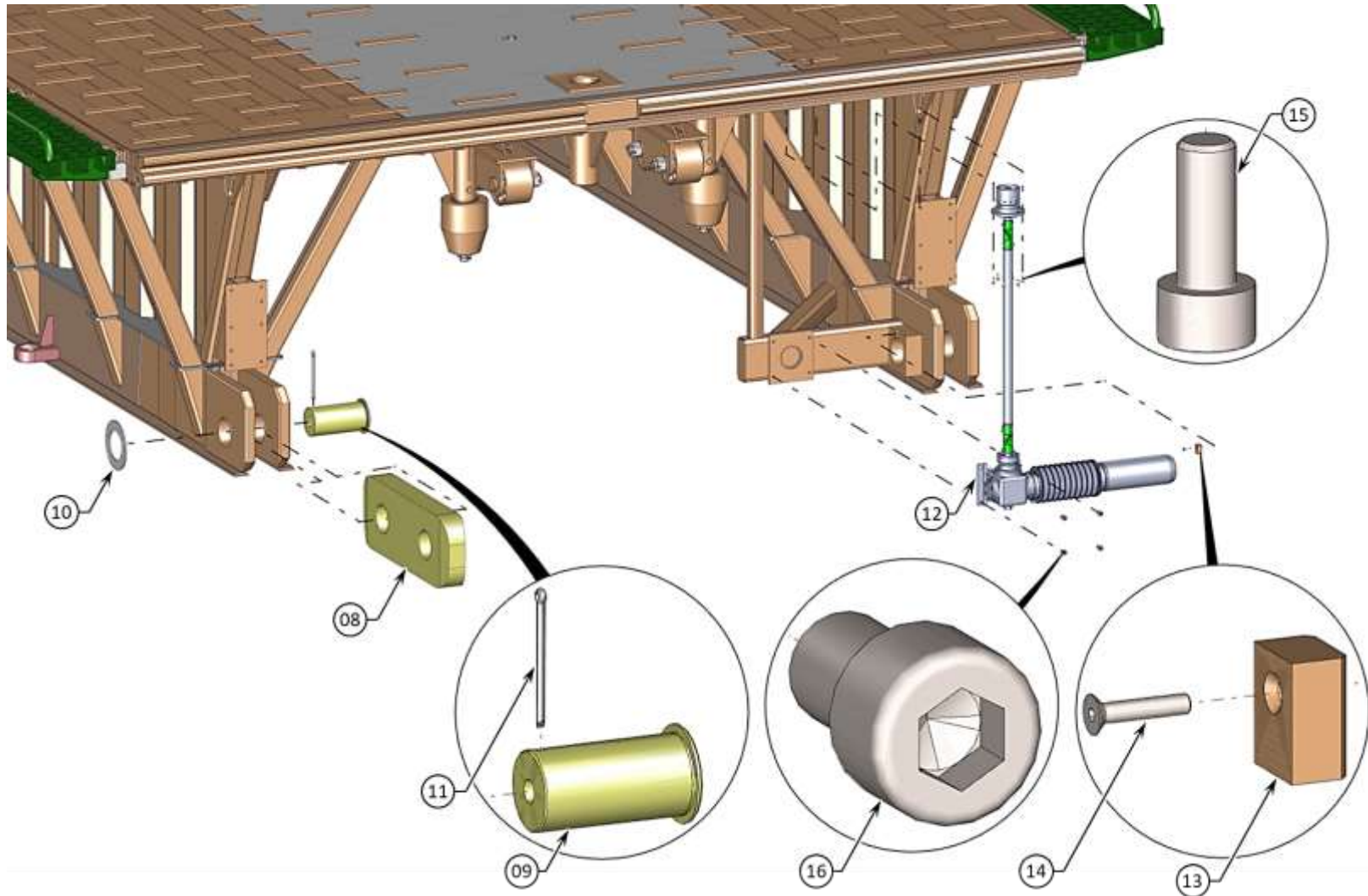
BRIDGE END MODULE ASSY - VIEW 2
