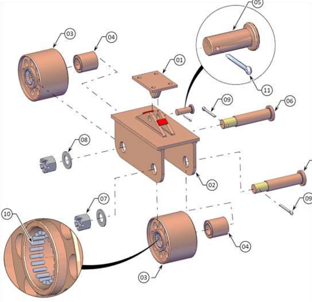
SUPPORT ROLLER ASSEMBLY (BCM) - VIEW 1
