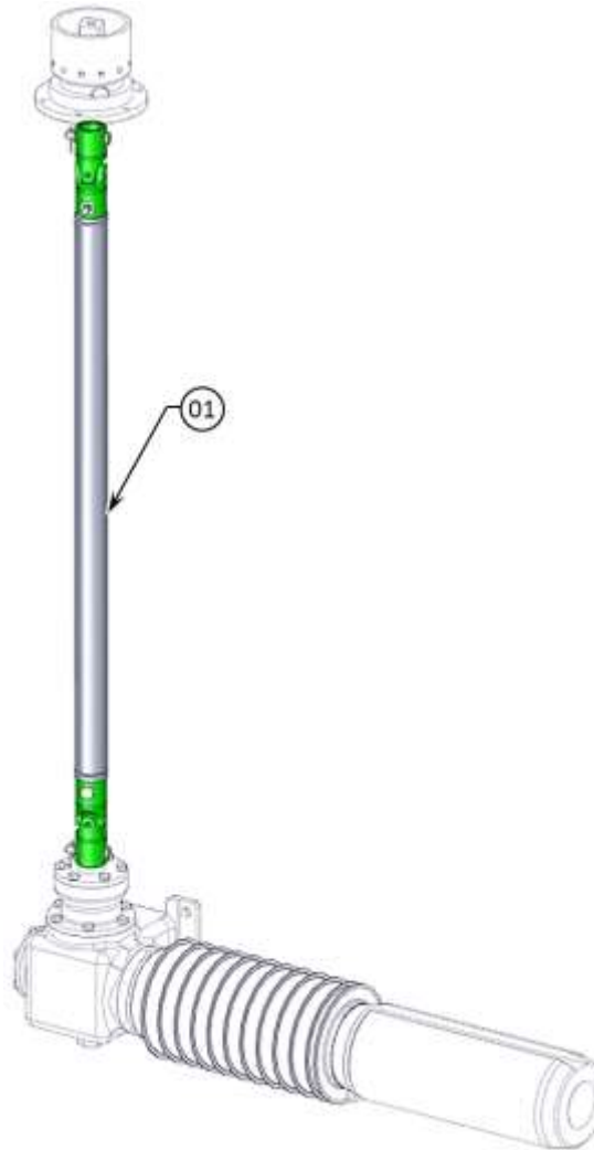
ASSEMBLY CONNECTING SHAFT (BRIDGE TO BRIDGE LOCKING MECHANISM)
