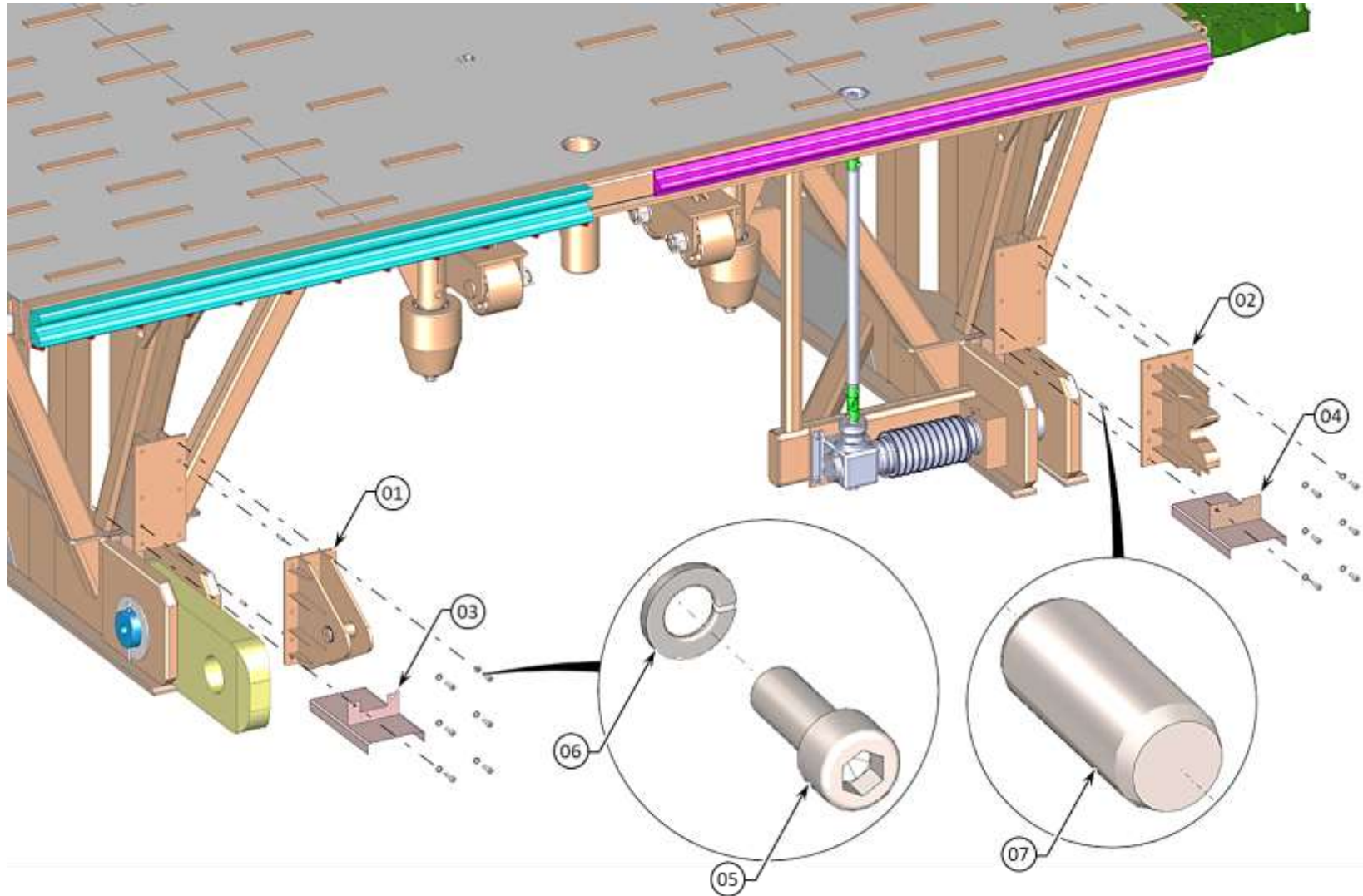
BRIDGE CENTRE MODULE ASSEMBLY - VIEW 1
