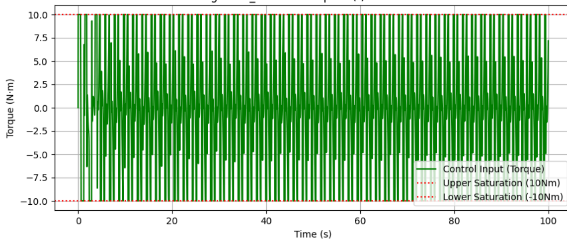
Fig 5-2-k_2: Control Input u(t) over Time
