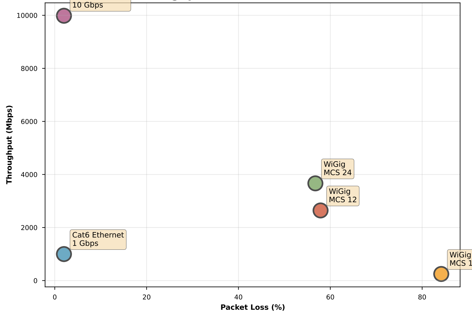
Throughput vs Packet Loss Trade-off
