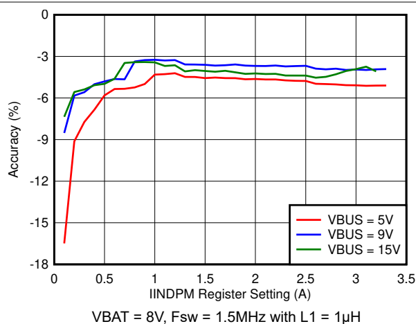
Figure 7-17. Input Current Regulation (IINDPM) Accuracy
