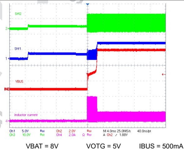
Figure 9-5. OTG Startup at 500-mA Load
