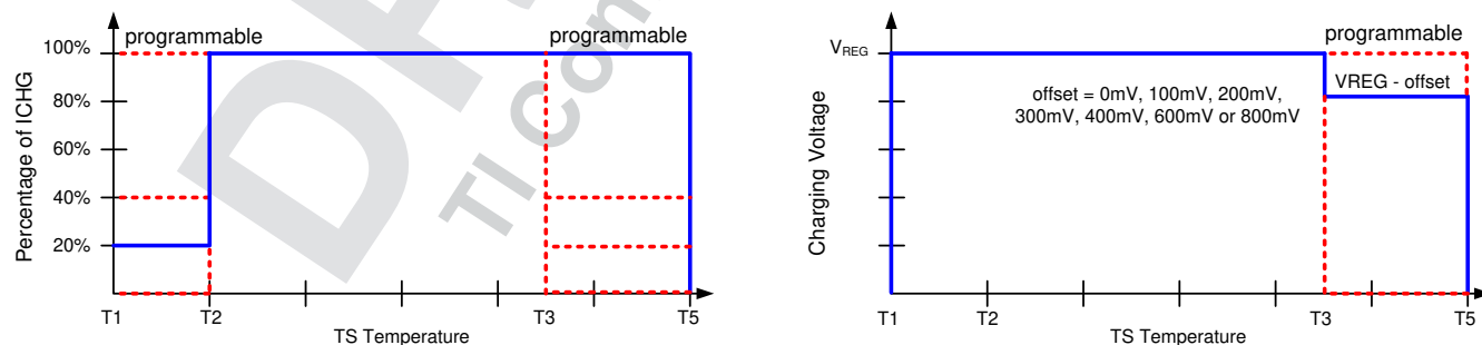
Figure 8-10. TS Charging Values
