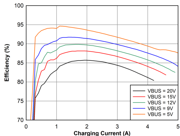
Figure 7-2. 1s Battery Charge Efficiency, 1.5 MHz
