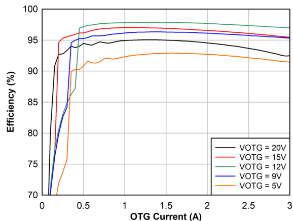
Figure 7-13. 3s Battery OTG Efficiency, 750 kHz
