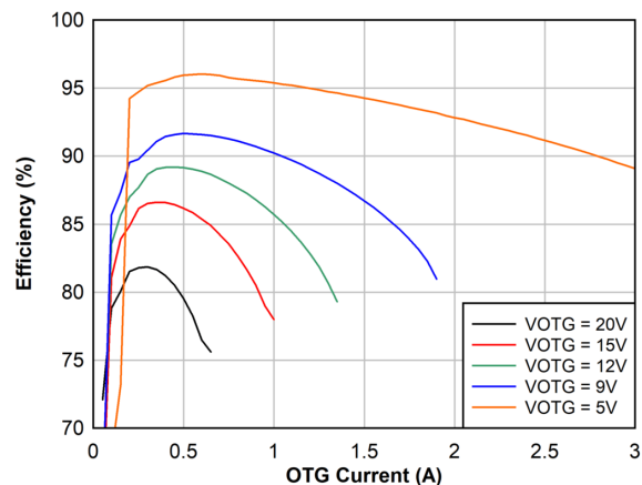
Figure 7-10. 1s Battery OTG Efficiency, 1.5 MHz
