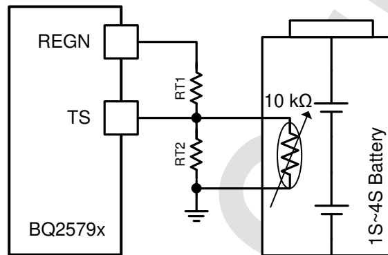
Figure 8-11. TS Resistor Network
