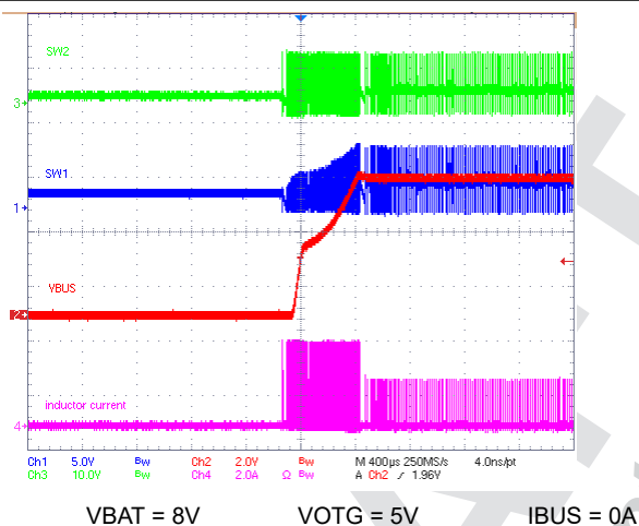
Figure 9-4. OTG Startup at No Load
