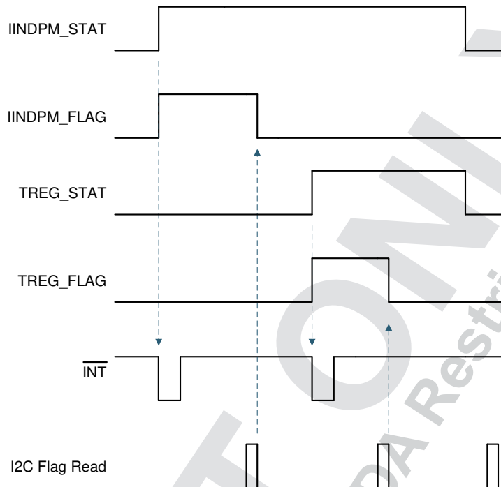
Figure 8-13. \overline{\text{INT}} Generation Behavior Example
