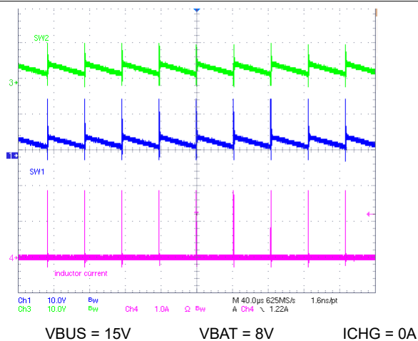
Figure 9-2. Buck Mode PFM with OOA
