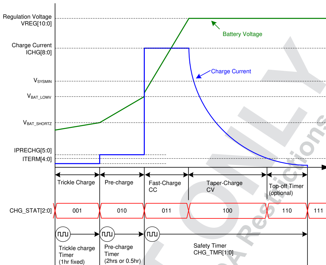
Figure 8-9. Battery Charging Profile
