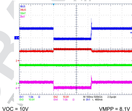
Figure 9-10. MPPT Operation Zoom
