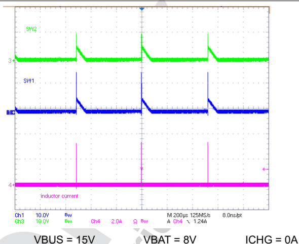
Figure 9-3. Buck Mode PFM without OOA
