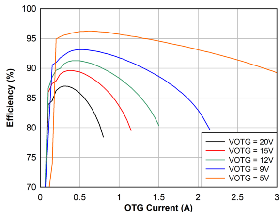
Figure 7-9. 1s Battery OTG Efficiency, 750 kHz
