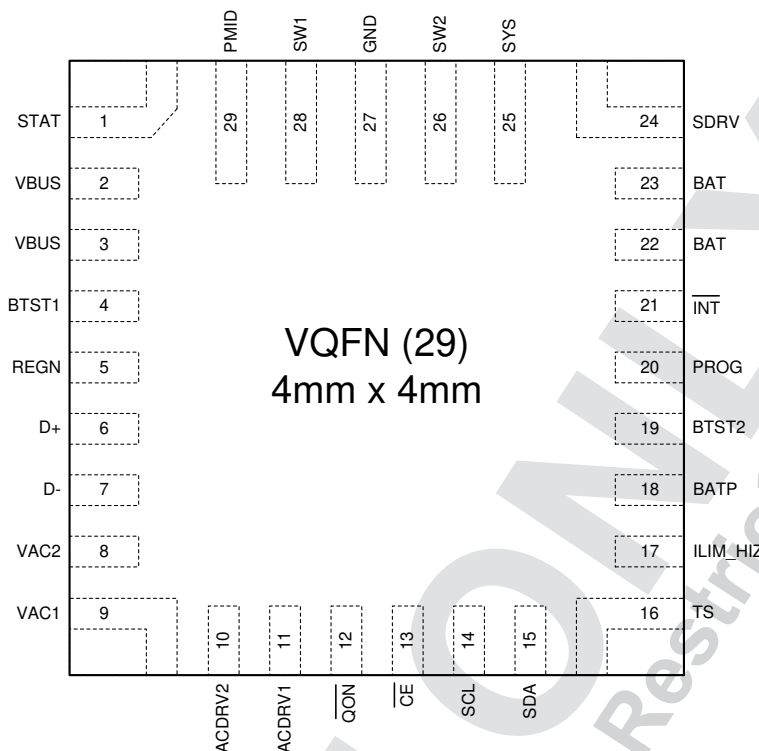
Figure 6-1. RQM Package 29-Pin VQFN Top View
