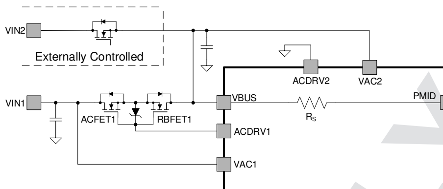
Figure 8-3. One ACFET-RBFET Structure Supporting One Input at VAC1 and/or One Input at VBUS
