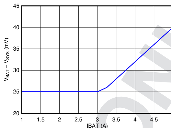
Figure 8-7. BATFET I-V Curve
