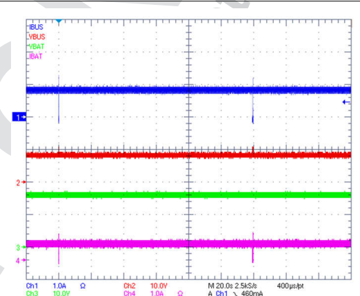
Figure 9-7. IINDPM Transient Response
