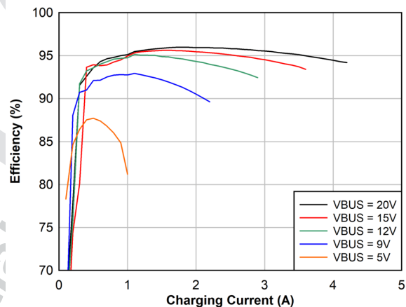
Figure 7-6. 3s Battery Charge Efficiency, 1.5 MHz
