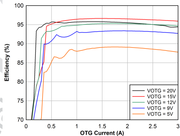
Figure 7-14. 3s Battery OTG Efficiency, 1.5 MHz
