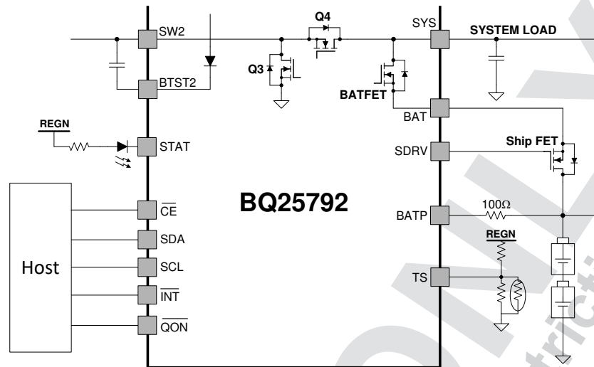
Figure 8-14. The Application Diagram for the External Ship FET
