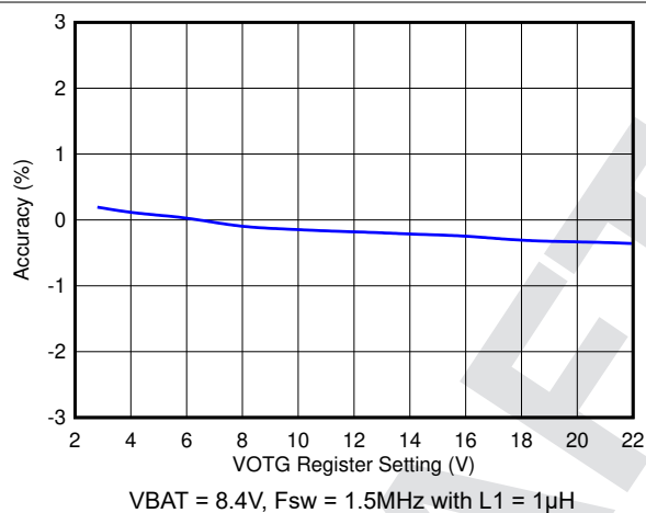
Figure 7-19. OTG Voltage Regulation (VOTG) Accuracy
