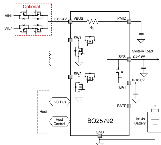
Simplified Schematic
