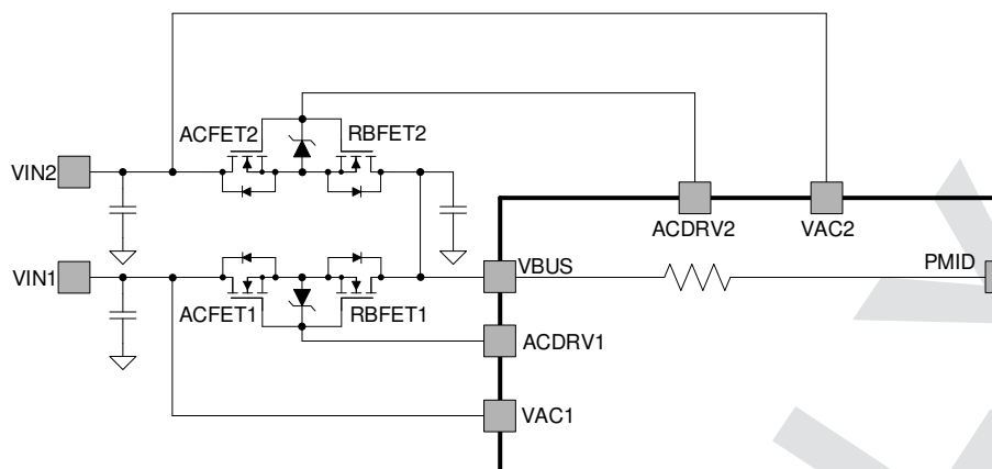
Figure 8-4. Two ACFETs-RBFETs Structure Supporting One Input at VAC1 and One Input at VAC2
