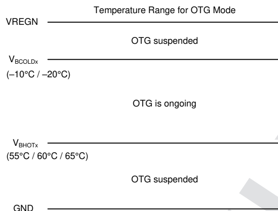
Figure 8-12. TS Pin Thermistor Sense Threshold in OTG Mode
