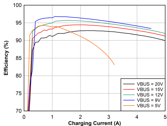
Figure 7-1. 1s Battery Charge Efficiency, 750 kHz
