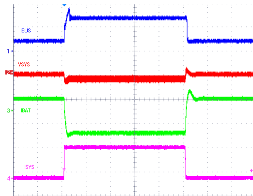
Figure 9-7. IINDPM Transient Response
