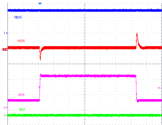
Figure 9-6. VSYS Load Transient Response
