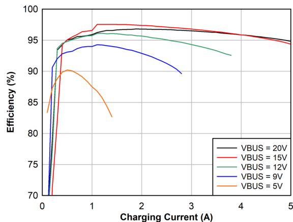
Figure 7-5. 3s Battery Charge Efficiency, 750 kHz
