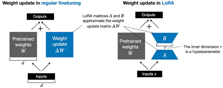
Figure 2.17: LoRA: Low-Rank Adaptation of frozen weight matrices [24]
