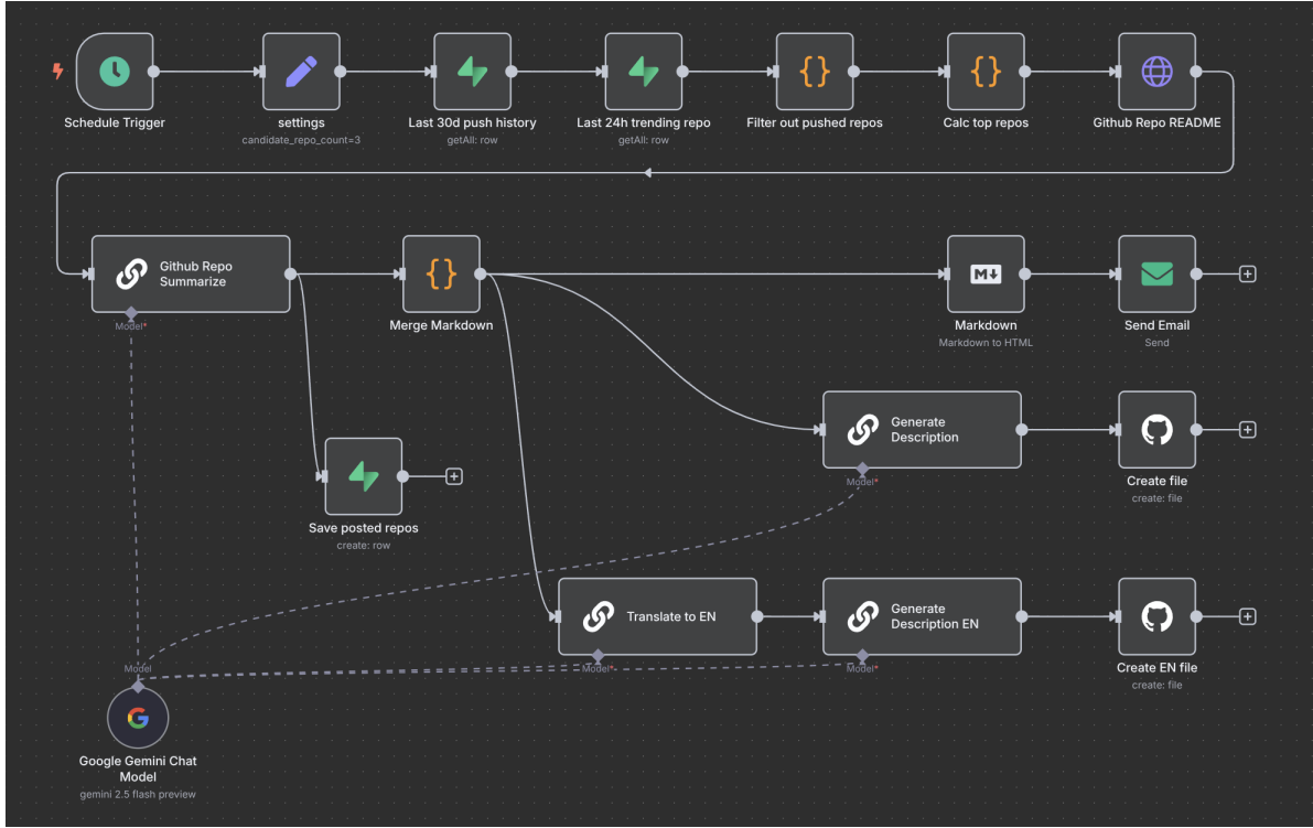
Figure 3.28: n8n Workflow: Automated Pipeline Orchestration [14]
