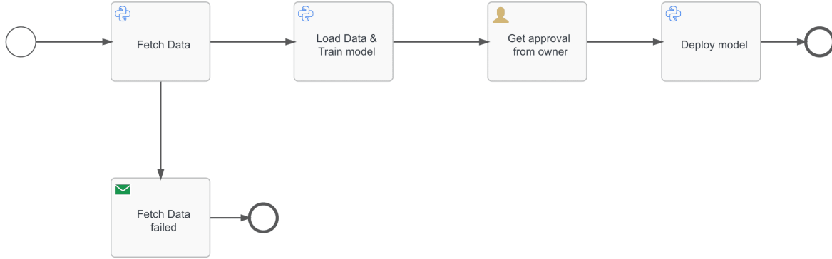
Figure 3.27: BPMN Diagram of the Offline Data Pipeline
