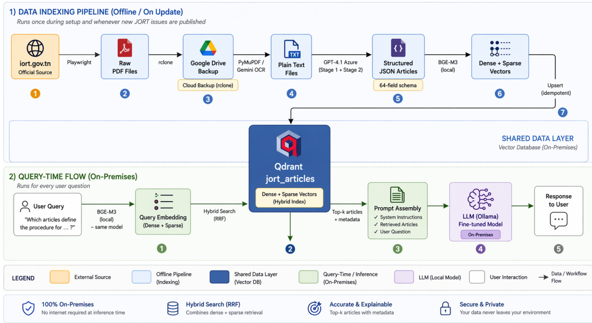
Figure 3.26: Overall Architecture of the Legal AI System
