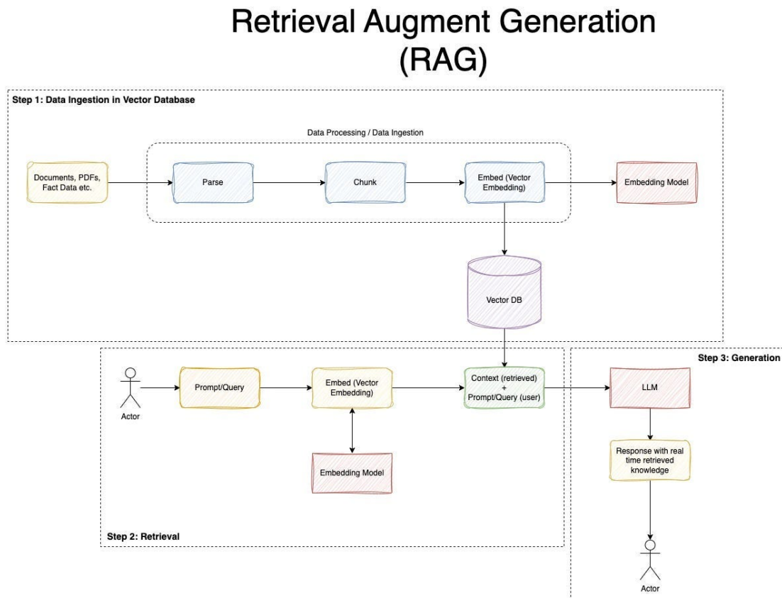
Figure 2.19: The RAG Pipeline: indexing, retrieval, and generation stages [28]
