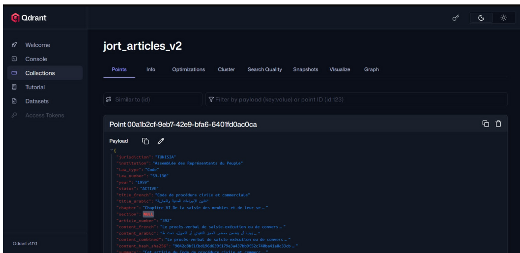
FIG. 4.42: Qdrant Dashboard Showing the jort_articles_v2 Collection After Indexing
