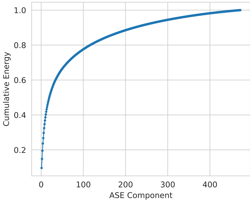
ASE Cumulative Energy (n = 472)
