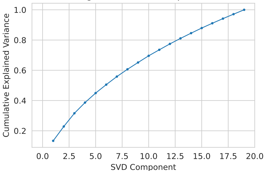
Singular Value Decomposition
