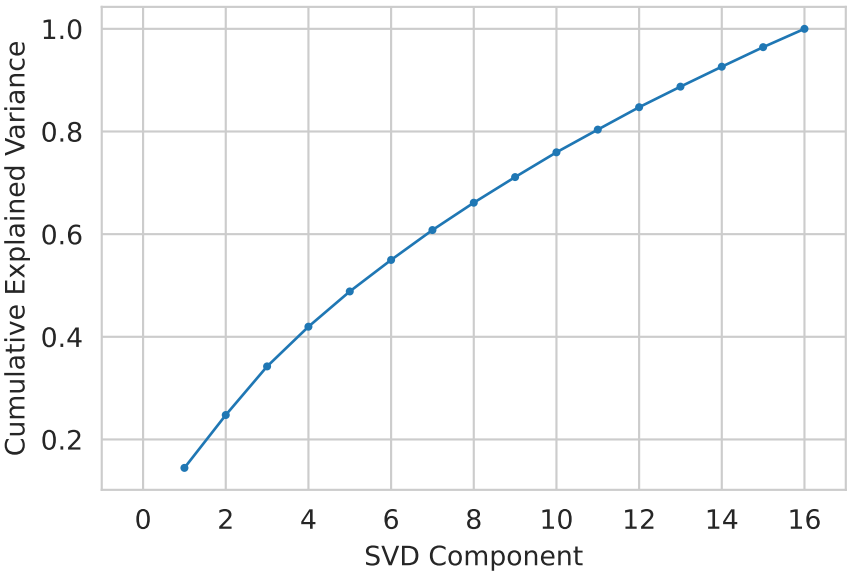
Singular Value Decomposition
