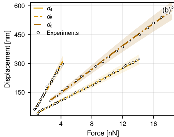
SonoVue force spectroscopy
