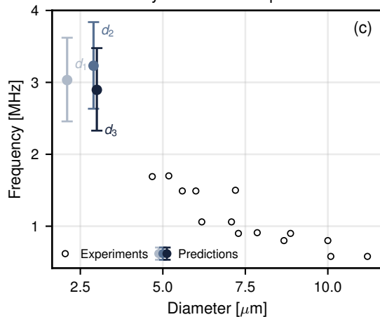
Definity resonance frequencies
