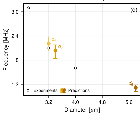
SonoVue resonance frequencies
