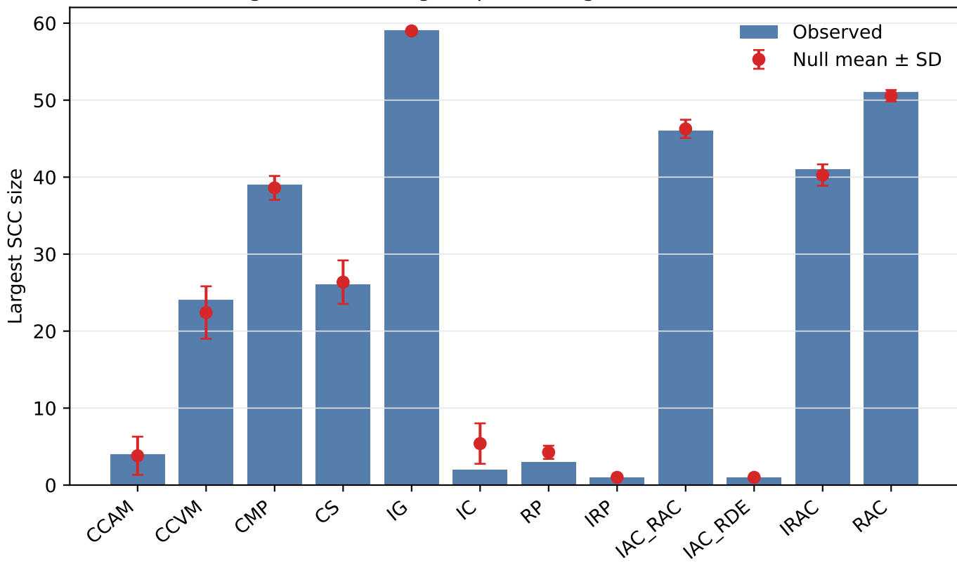
Largest SCC vs degree-preserving null (10000 draws)
