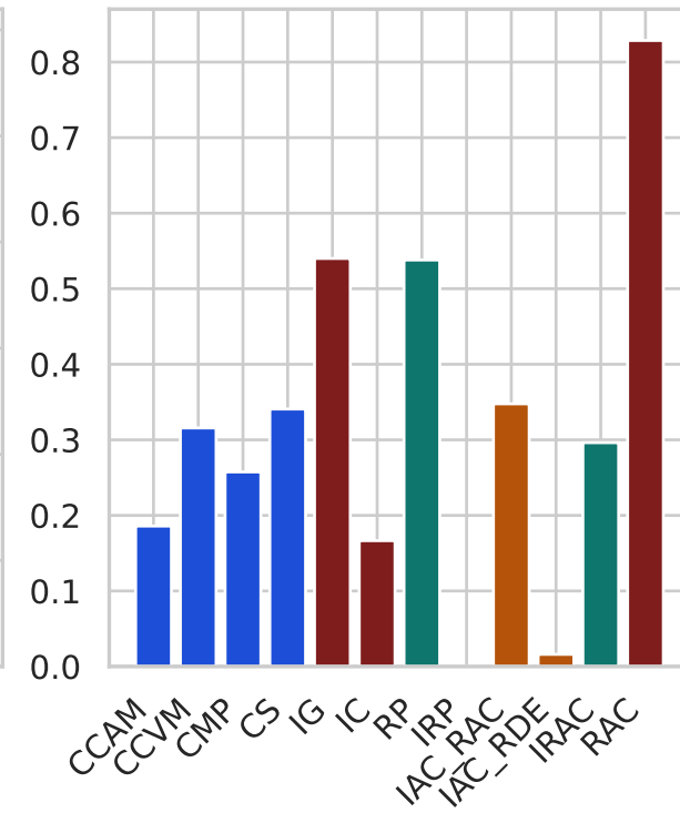
Undirected clustering
