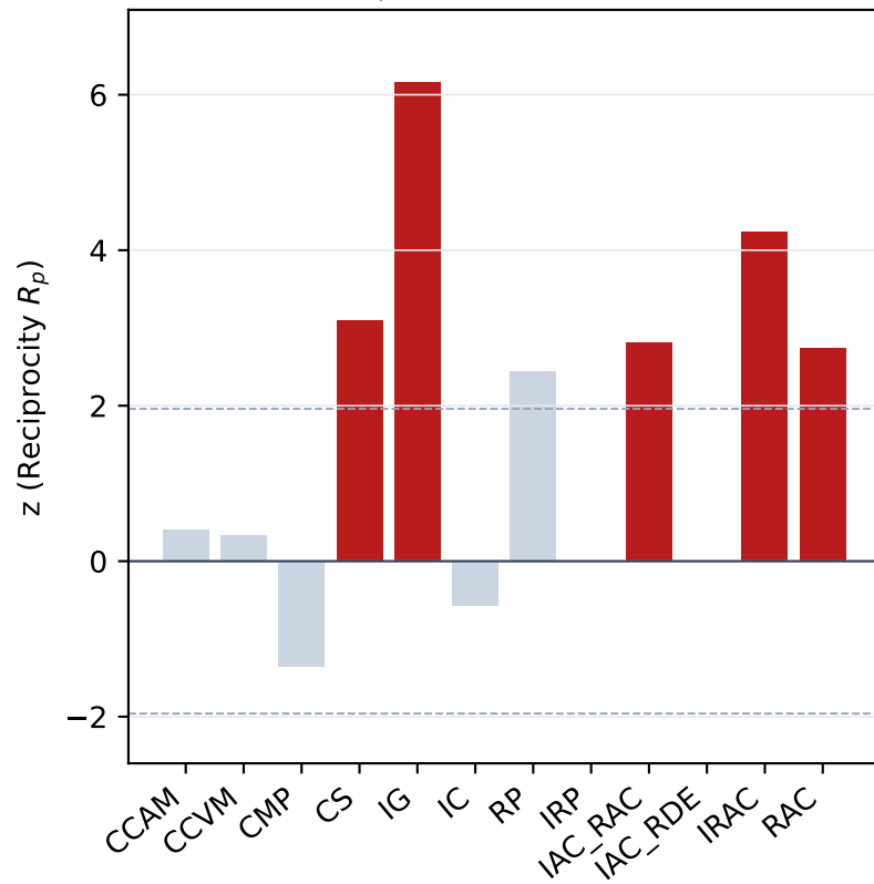
Reciprocity R_p vs degree-preserving null
