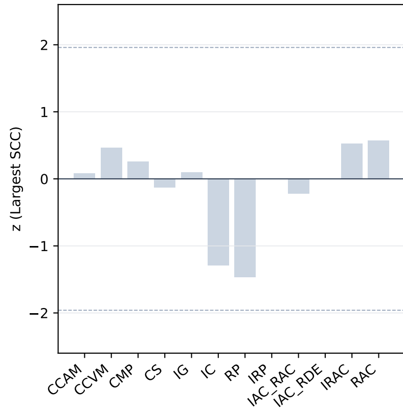
Largest SCC vs degree-preserving null
