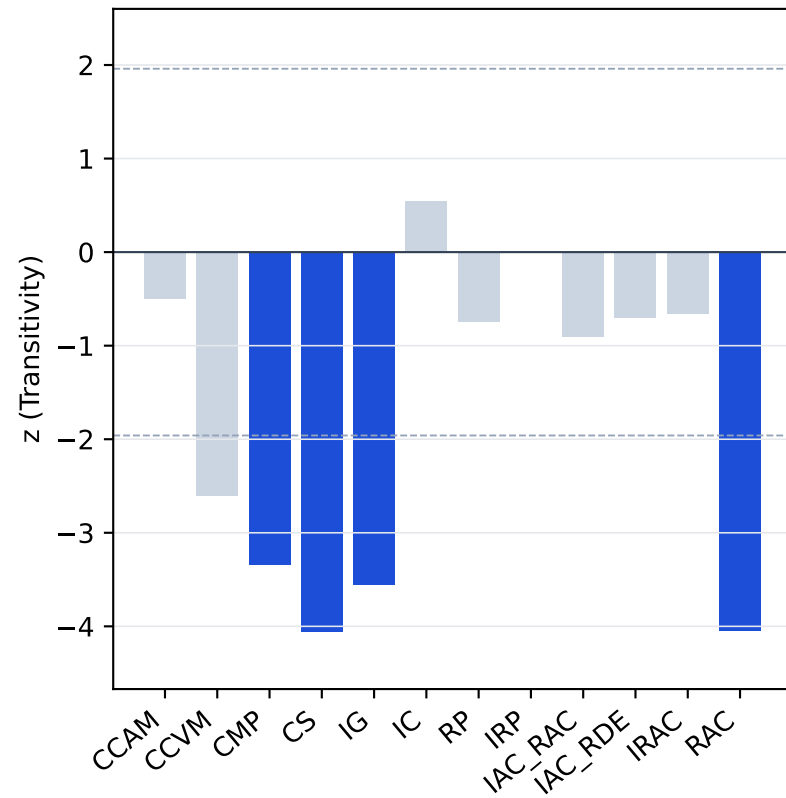
Transitivity vs degree-preserving null
