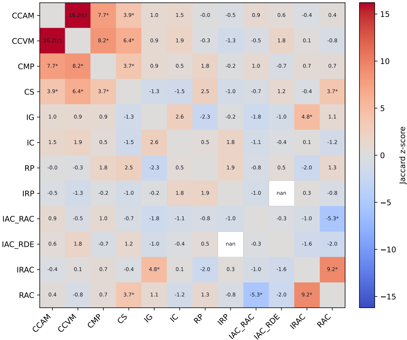
Jaccard overlap vs degree-preserving null (BY-FDR)
