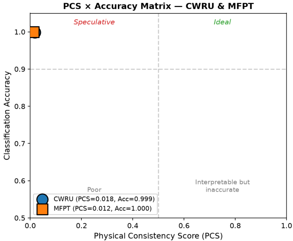
Figure 10: PCS × Accuracy matrix — CWRU & MFPT combined
