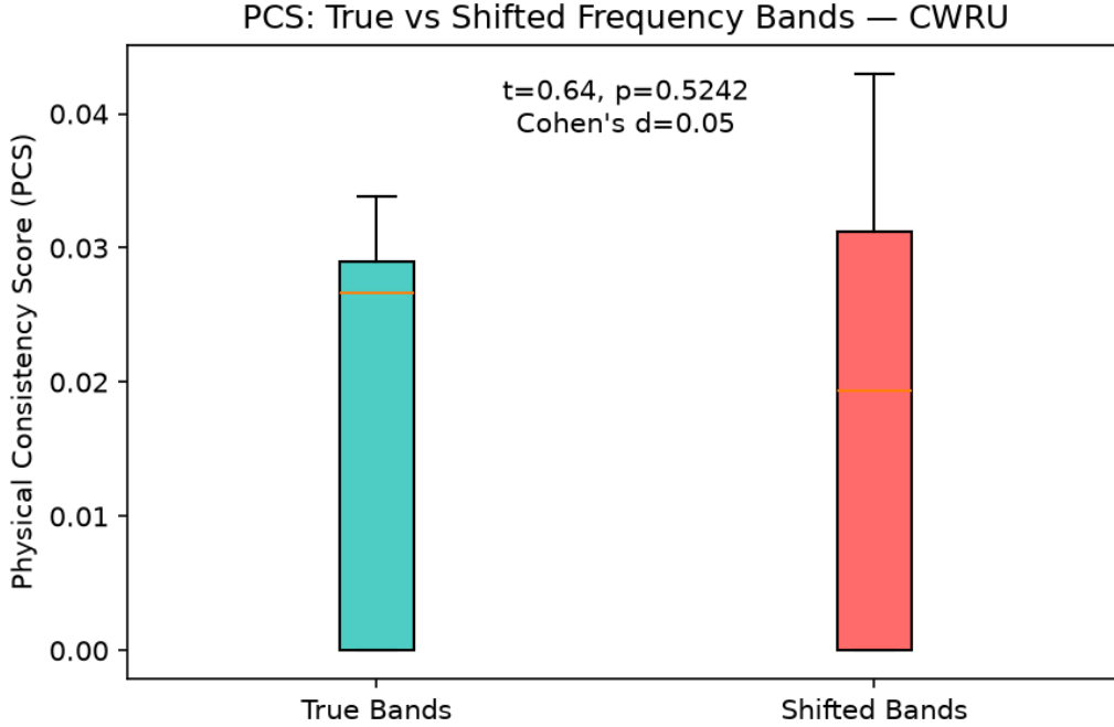
Figure 3: Box plot of PCS for true versus shifted frequency bands on CWRU
