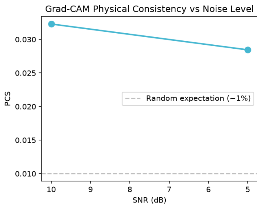
Figure 5: PCS as a function of SNR on CWRU
