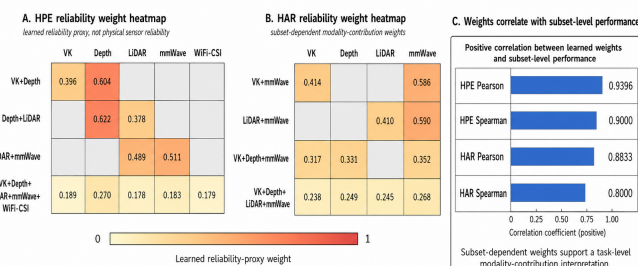
Learned Reliability-Proxy Weights Across Modality Subsets
