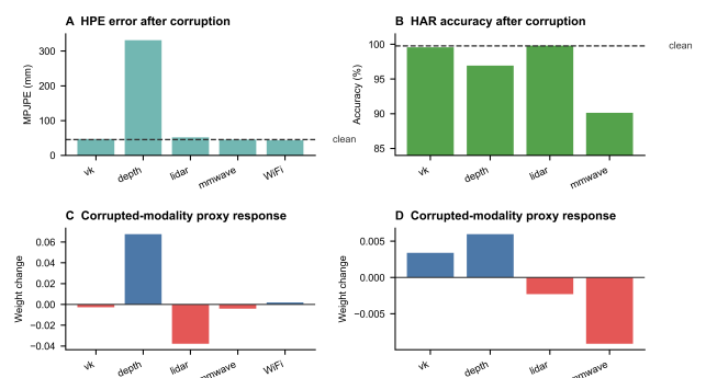
Reliability-aware proxy under synthetic modality corruption
