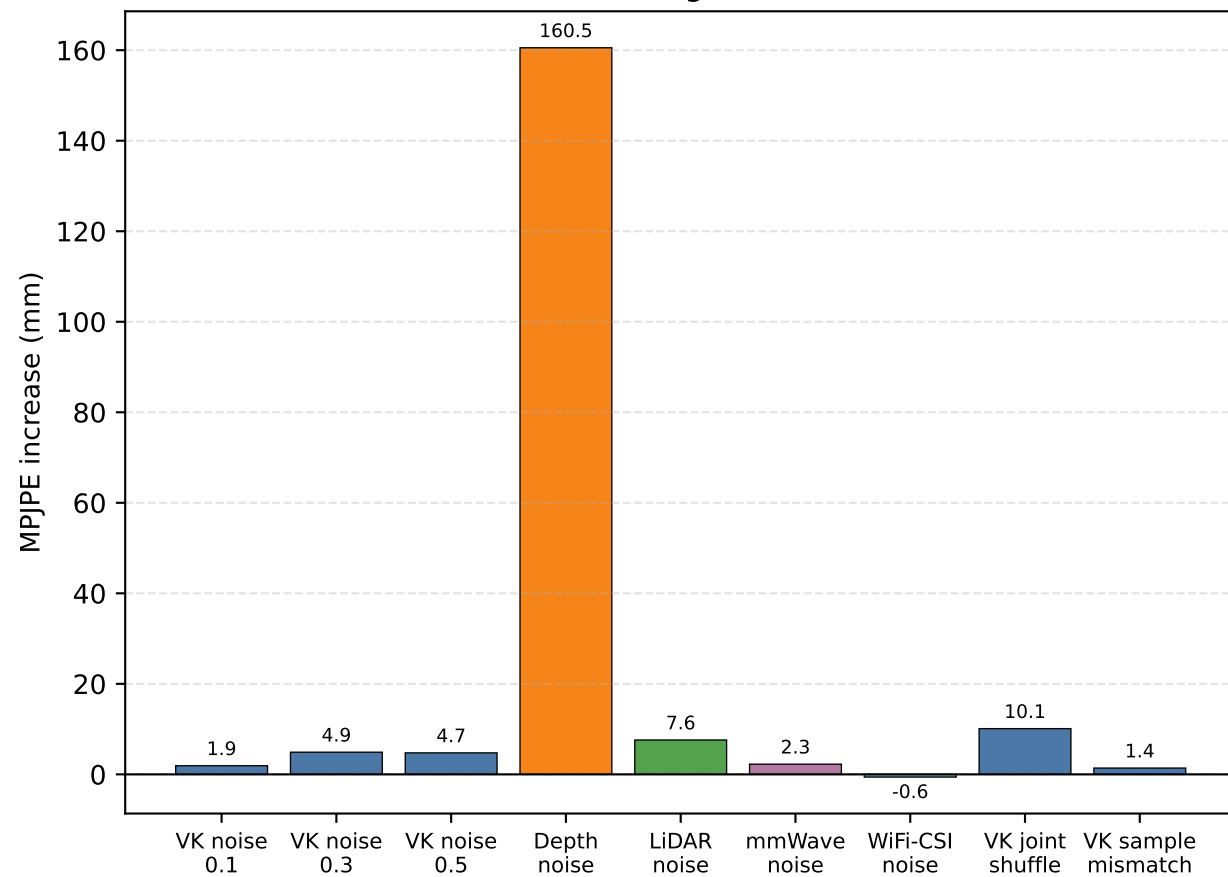
HPE diagnostic
