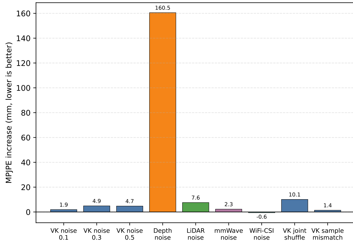
HPE: degradation under semantic and sensor perturbations
