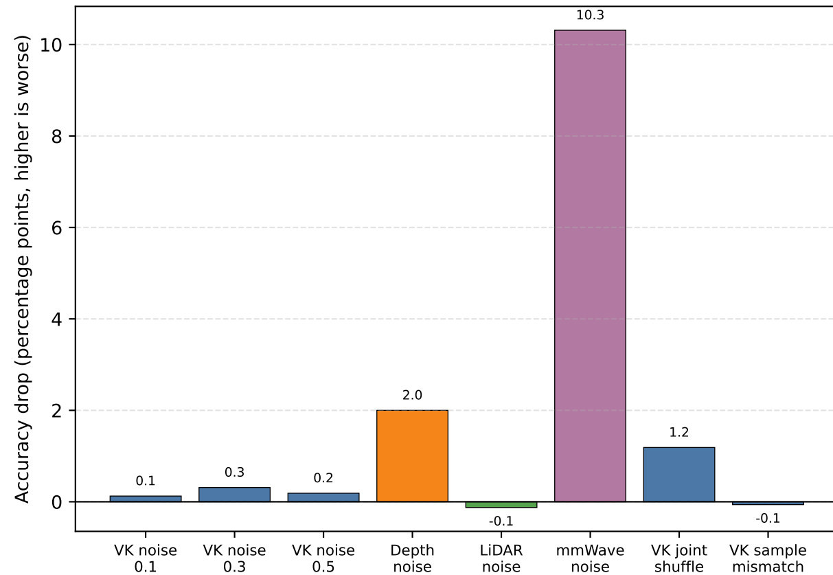
HAR: degradation under semantic and sensor perturbations
