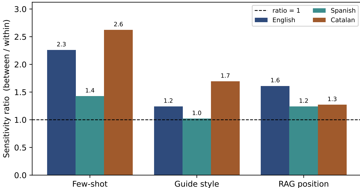
Prompt sensitivity per axis, by language (noise floor = 0.23)
