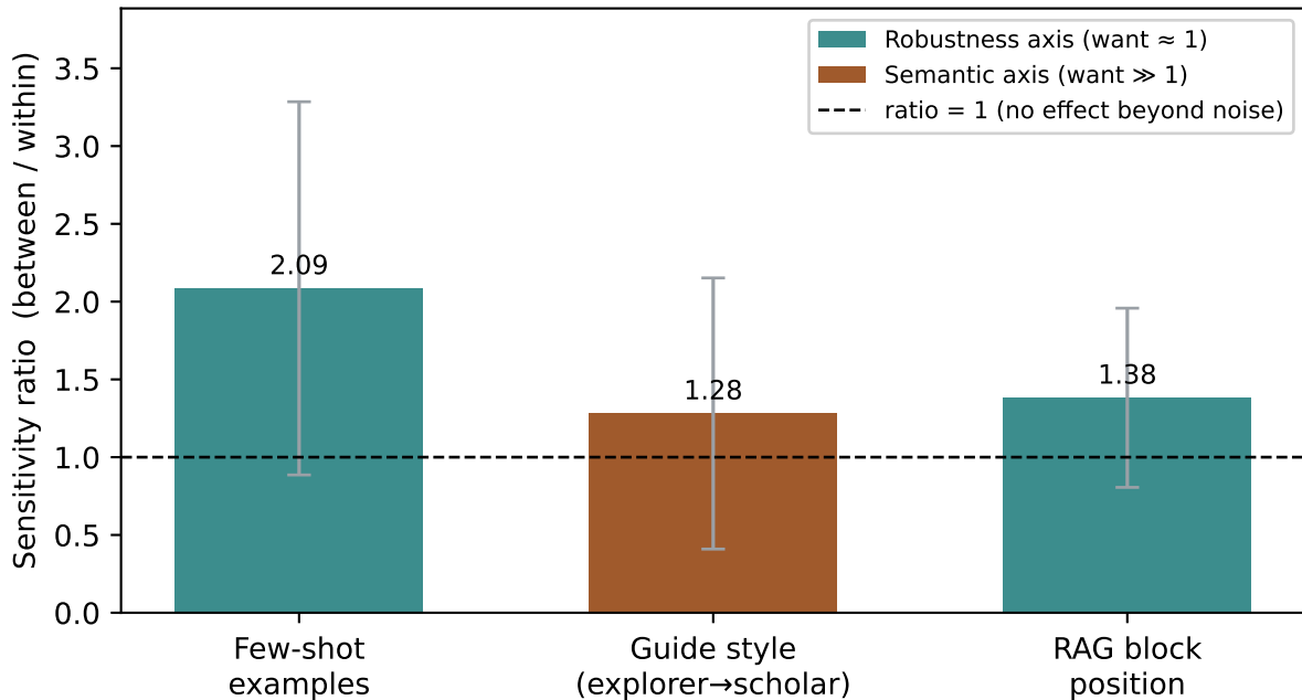
Prompt sensitivity per axis (noise floor = 0.23; 12 items \times 3 langs \times 3 runs)
