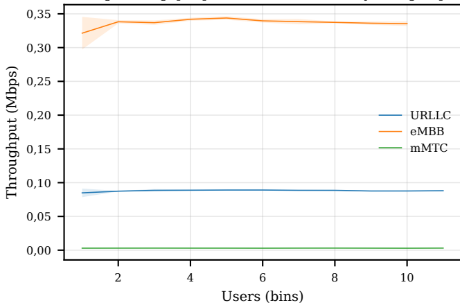
Average throughput per scenario (95% CI) (by user groups)
