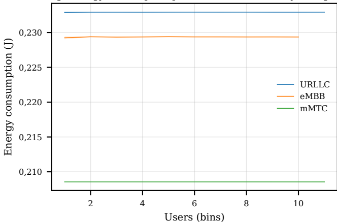
Average energy consumption per scenario (95% CI) (by user groups)
