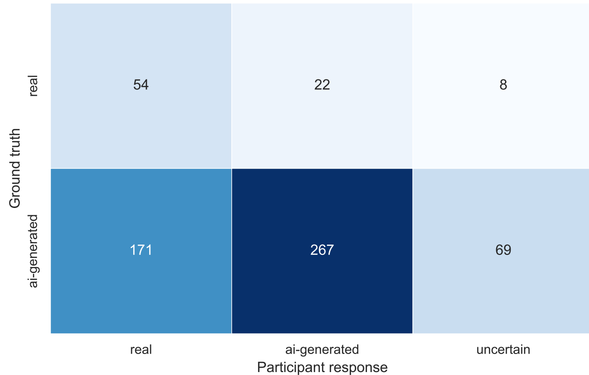
Confusion Matrix (counts)
