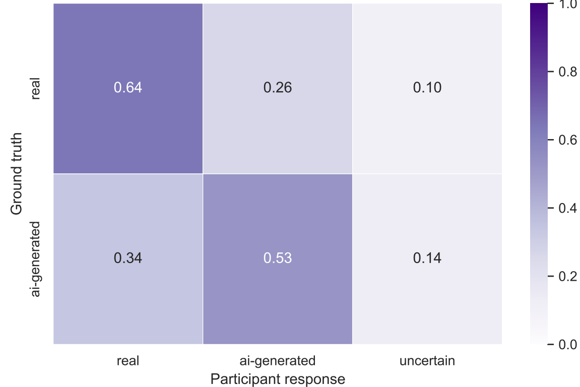
Confusion Matrix (row-normalized proportions)
