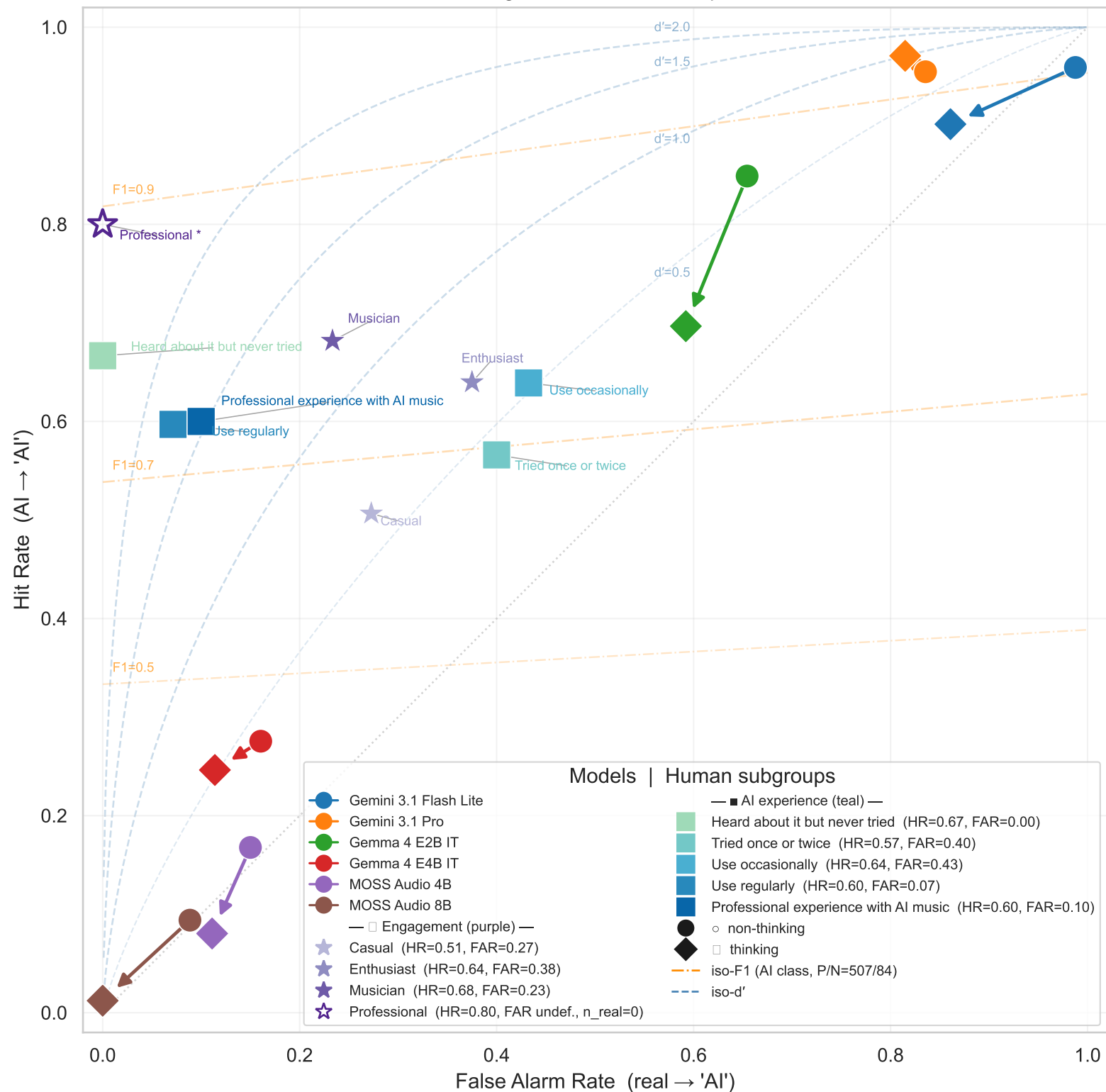
Thinking Mode Effect: ROC Space
