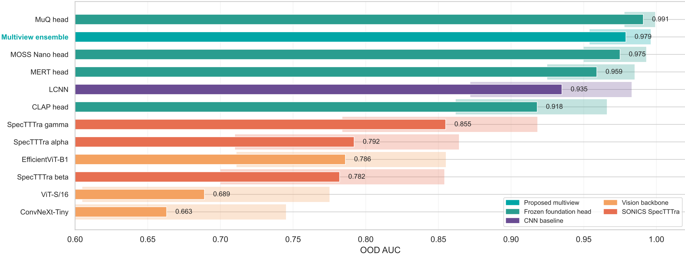
A. Detector head-to-head on out-of-distribution generators
