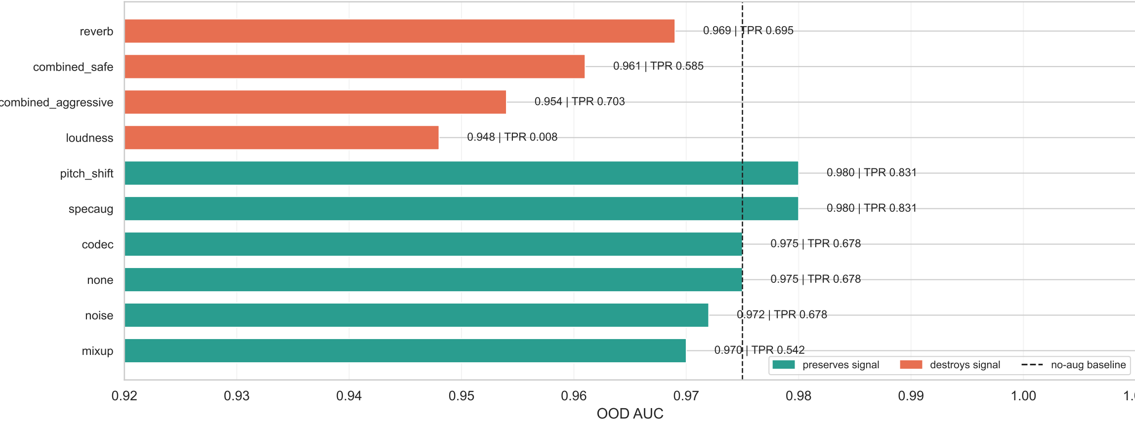
C. LCNN augmentation ablation
