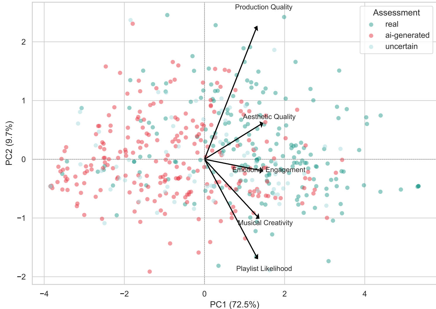
PCA Biplot of Rating Dimensions
