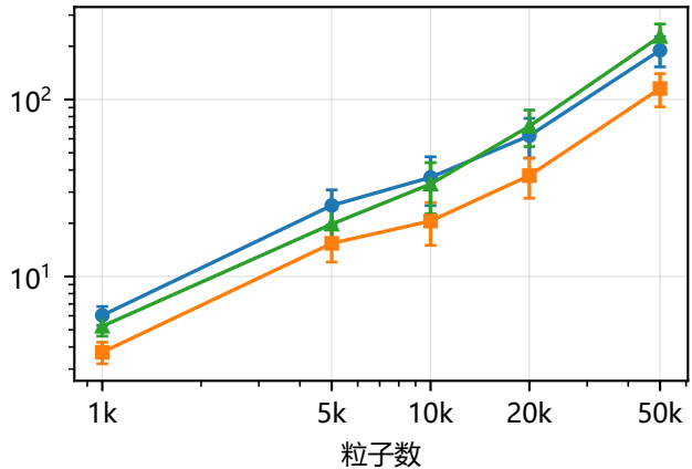
PCISPH
