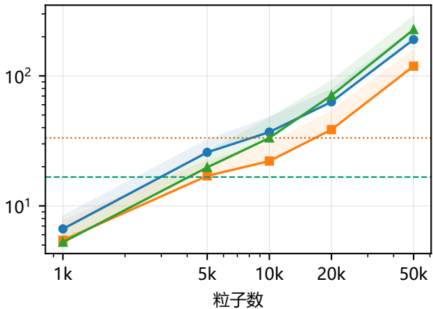
PCISPH
