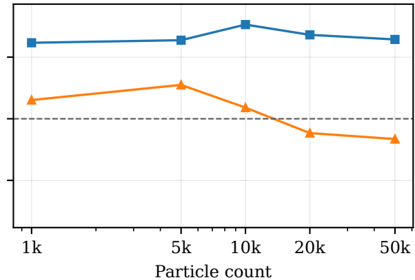
PCISPH
