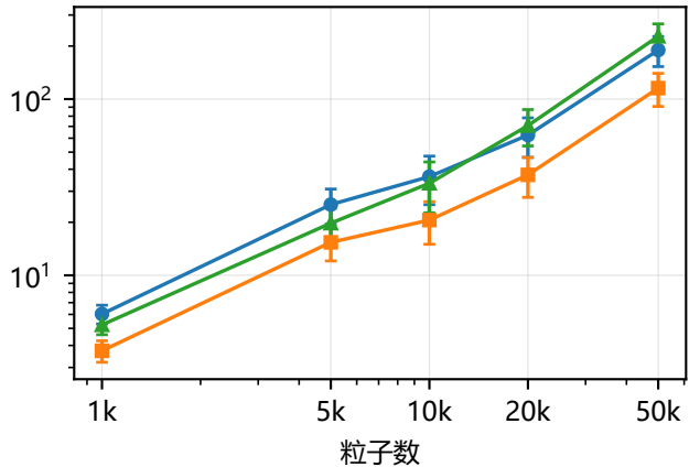
PCISPH
