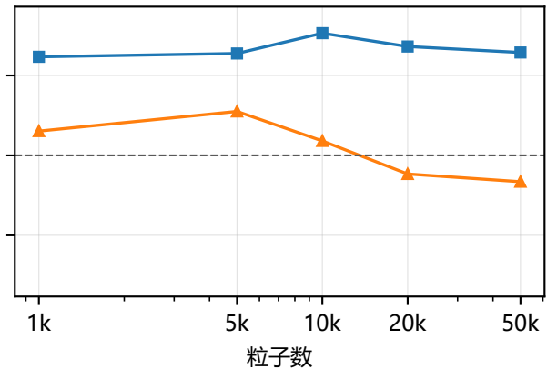
PCISPH
