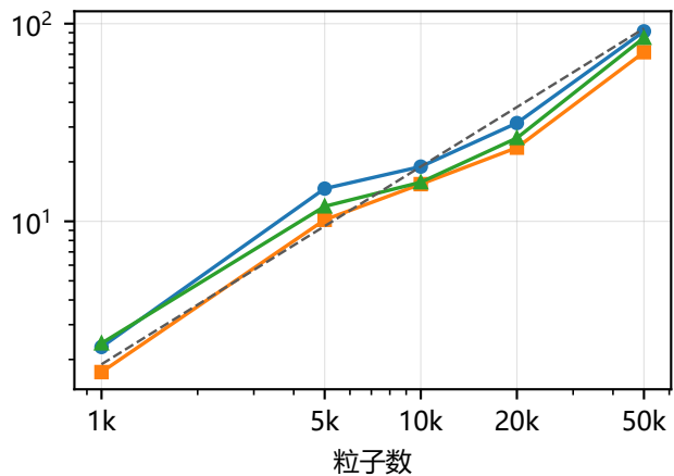
PCISPH
