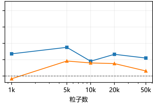
PCISPH
