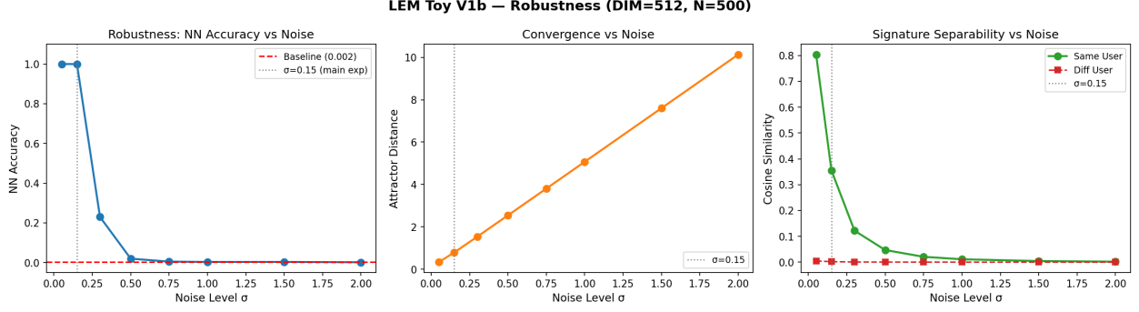
Figure 2: Robustness of LEM signatures to noise \sigma . Left: NN accuracy with phase transition at \sigma \approx 0.25 . Centre: attractor distance (linear in \sigma ). Right: cosine separability collapse.
